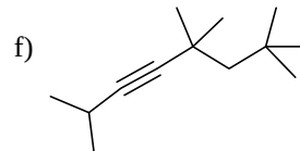
2,5,5,7,7-pentamethyl-3-octyne
