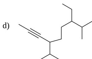
7-ethyl-4-(1-methylethyl)-8-methyl-2-nonyne
