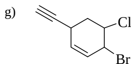
3-bromo-4-chloro-6-ethynylcyclopentene
