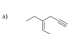
Z-3-ethyl-2-hexen-5-yne
