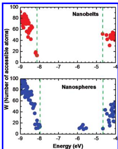
Figure 4. Number of accessible atoms ( W ) for each electronic state near the valence and conduction band edges of the nanobelts and nanospheres. Note that the smaller the W , the more localized the state. The dashed lines indicate the valence and conduction band edges.
