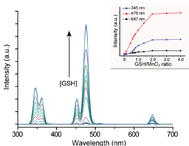
Figure 2. Photoluminescence response of \text{MnO}_2 -modified \text{NaYF}_4\text{:Yb/Tm@NaYF}_4 nanoparticles as a function of GSH concentration (0–10 mM) in an aqueous solution. (Inset) Plot of luminescence intensity at 345, 476, and 647 nm, respectively, against the GSH/ \text{MnO}_2 molar ratio. The spectra were recorded under excitation of a 980-nm laser at a power density of 10\text{ W cm}^{-2} .
