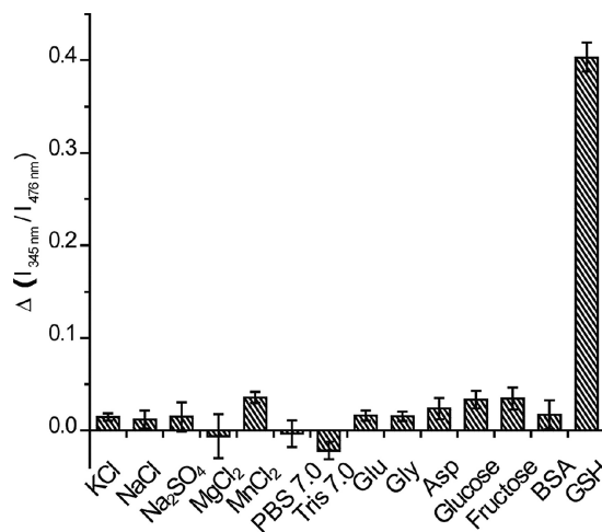
Figure 3. Photoluminescence response of \text{MnO}_2 -modified \text{NaYF}_4\text{:Yb/Tm@NaYF}_4 nanoparticle solutions in the presence of different electrolytes and biomolecules (0.1 M each; for bovine serum albumin: 1\text{ mg/mL} ). The photoluminescence response was evaluated by calculating the change in the relative luminescence intensity ratio ( I_{345\text{nm}}/I_{476\text{nm}} ) of \text{MnO}_2 -modified nanoparticles.
