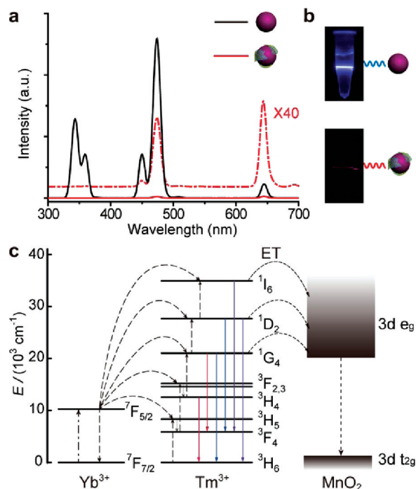
Figure 1. (a) Upconversion emission spectra of core–shell \text{NaYF}_4\text{:Yb/Tm@NaYF}_4 nanoparticles (black line) and \text{MnO}_2 -modified nanoparticles with a UCNP/ \text{MnO}_2 molar ratio of 1:0.25 (red lines). The dotted line, enhanced 40 times, reveals the higher emission intensity at 645 nm relative to that at 476 nm. (b) Corresponding photographs of UCNP (top) and \text{MnO}_2 -modified UCNP (bottom) solutions under the 980 nm excitation. (c) Proposed excitation and energy-transfer mechanisms in \text{MnO}_2 -modified UCNP. Note that the samples in (a) and (b) were dispersed in deionized water, and the concentrations of lanthanide ions were adjusted to 0.01 M. The emission spectra and photographs were recorded with a diode 980-nm laser at a power density of 10\text{ W cm}^{-2} .
