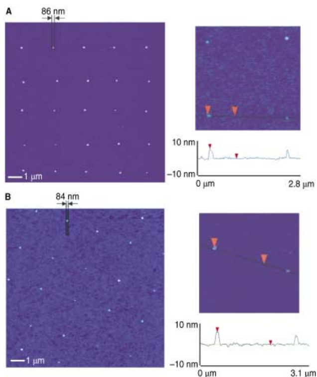
Figure 3. Protein nanoarrays of A) ubiquitin and B) thioredoxin. Images were taken at 0.5 Hz in tapping mode (Nanoscope IIIa and multimode microscope from Digital Instruments). The contact time was 3 s for the ubiquitin array and 5 s for the thioredoxin array.
