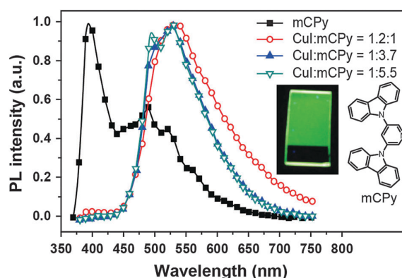
Fig. 11 Photoluminescence spectra of a neat mCPy film (at 77 K) and CuI:mCPy films with different ratios at room temperature under excitation at 350 nm (inset: photographic image of a CuI:mCPy film excited at 365 nm using a UV lamp). (Reproduced with permission from ref. 62. Copyright 2011, American Chemical Society.)
