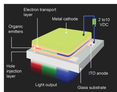
Fig. 4 Device structures of prototype sandwich-structured OLEDs.
