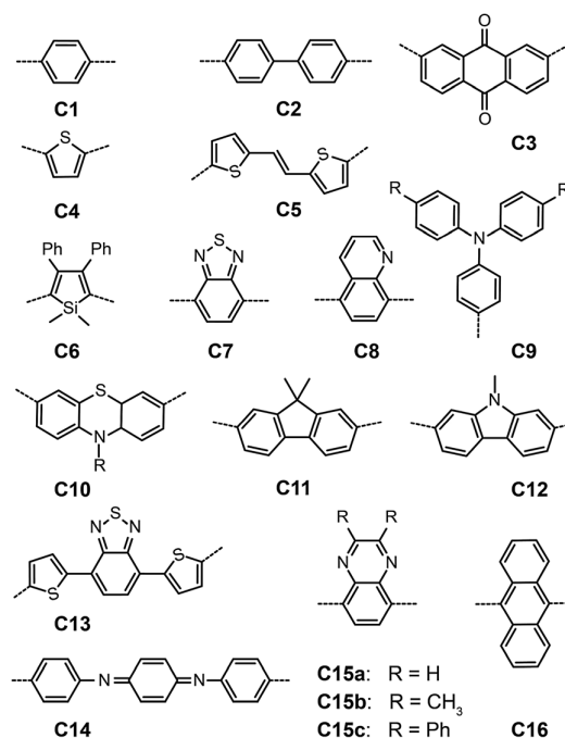
Fig. 25 Conventional building blocks for OPVs.
