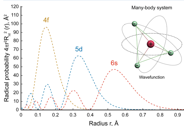
Figure 8. Radial parts of the wave functions for Ce (4f, 5d, and 6s) atomic orbitals. The vertical axis represents the probability of finding an electron at a distance of r from the nucleus. The inset depicts complex many-body interactions (electron–electron interactions in solid green lines and electron–nucleus interactions in solid lines with a mixed color of green and red). The dotted gray circles indicate the schematic wave function of orbitals. Adapted from ref 168. Copyright 1964 American Chemical Society.
