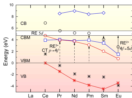
Figure 12. Representative energy levels of a series of divalent and trivalent rare-earth (RE) ions when doped in \text{LaSi}_3\text{N}_5 host lattice. * and \circ labels refer to the occupied and unoccupied 4f states of \text{RE}^{3+} , respectively. \square and \diamond labels refer to the occupied and unoccupied 4f states of \text{RE}^{2+} , respectively. Note that gray-colored circle and asterisk symbols stand for the experimentally observed 4f ground states. The dashed and solid arrows indicate charge transfer to trivalent lanthanides and f-d transition in divalent lanthanides, respectively. Adapted with permission from ref 283. Copyright 2015 Elsevier B. V.
