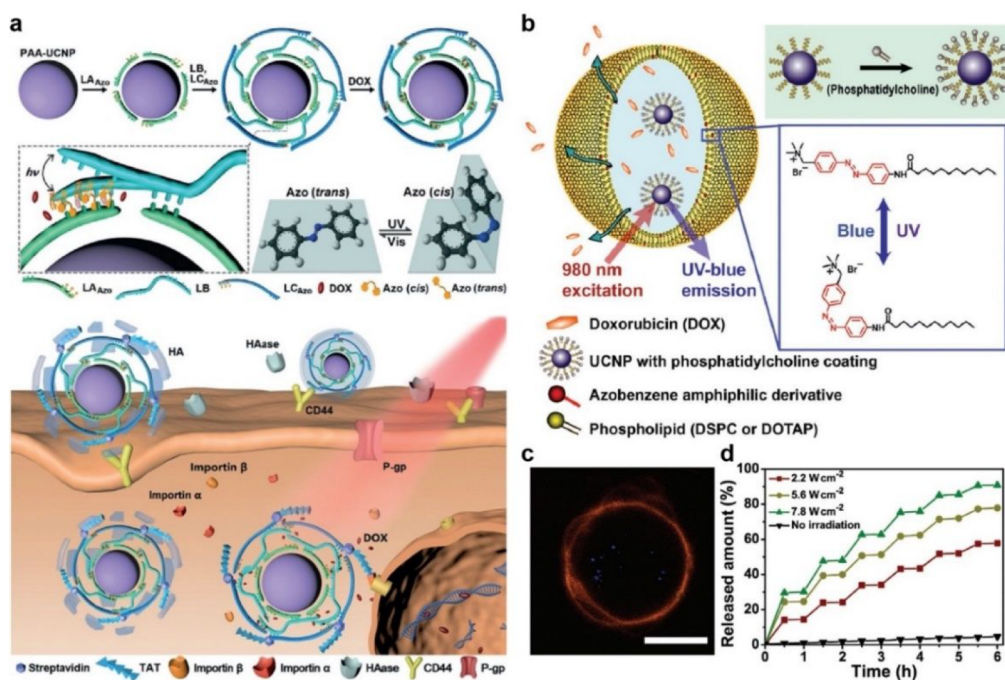
Figure 22. (a) Schematic of UCNP- \text{LA}_{\text{Azo}}\text{BC}_{\text{Azo}}/\text{DOX} assembly and NIR-triggered drug release in living cells. (b) Schematic of NIR-triggered drug delivery using azobenzene-liposome/UCNP hybrid vesicles. (c) Confocal cross sections of azobenzene-liposome/UCNP/CdSe hybrid vesicles. The scale bar is 5 \mu\text{m} . (d) Power-dependent drug release curves in buffer under intermittent irradiation with 980 nm light (Adapted with permission from refs 693 and 694. Copyright 2016 and 2019 Wiley-VCH Verlag GmbH & Co. KGaA, Weinheim).
