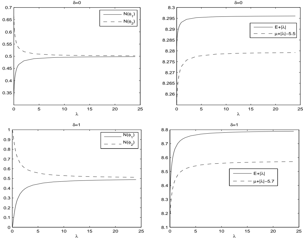
Figure 4: Mass of each component N(\phi_j) = \|\phi_j\|^2 ( j = 1, 2 ), energy E := E(\Phi_g) and chemical potential \mu := \mu(\Phi_g) of the ground states in Example 1 when \beta = 100 and \delta = 0, 1 for different \lambda .
