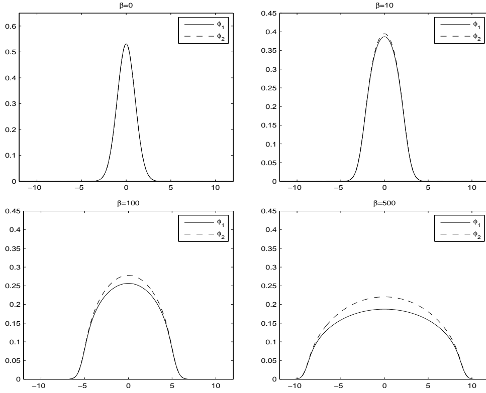
Figure 1: Ground states \Phi_g = (\phi_1, \phi_2)^T in Example 1 when \delta = 0 and \lambda = -1 for different \beta .
