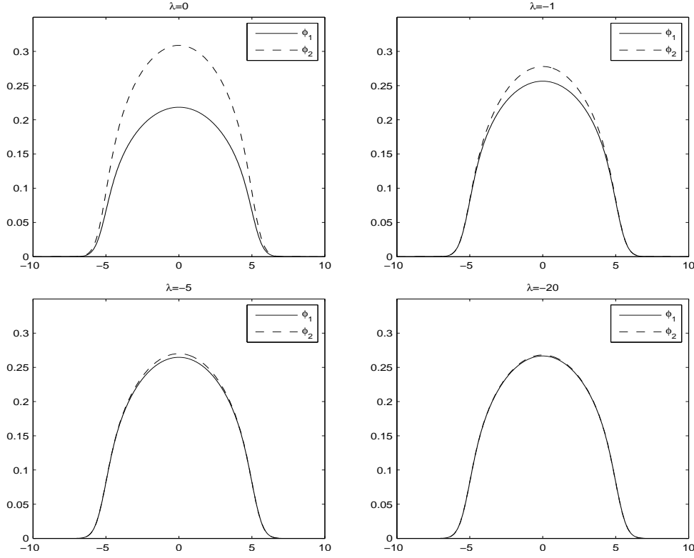
Figure 2: Ground states \Phi_g = (\phi_1, \phi_2)^T in Example 1 when \delta = 0 and \beta = 100 for different \lambda .
