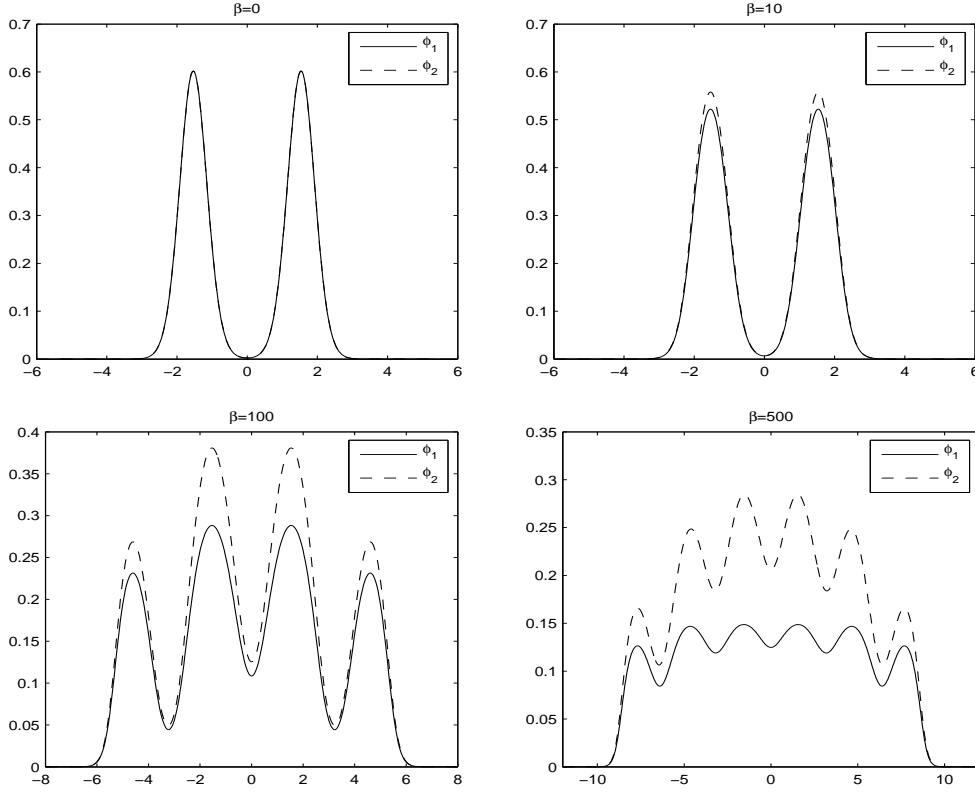
Figure 6: Ground states \Phi_g = (\phi_1, \phi_2)^T in Example 2 when \delta = 0 and \lambda = -1 for different \beta .
