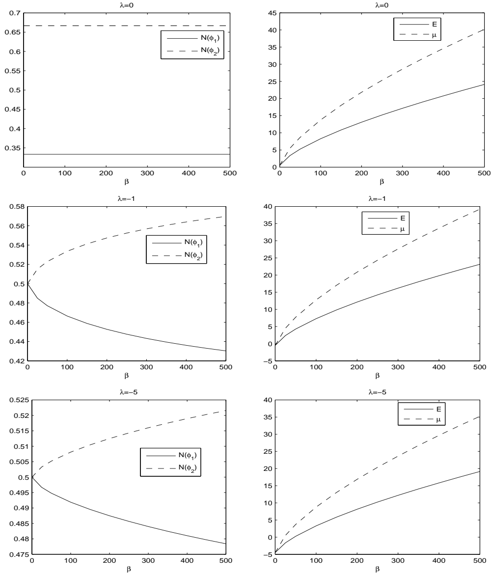
Figure 3: Mass of each component N(\phi_j) = \|\phi_j\|^2 ( j = 1, 2 ), energy E := E(\Phi_g) and chemical potential \mu := \mu(\Phi_g) of the ground states in Example 1 when \delta = 0 for different \lambda and \beta .
