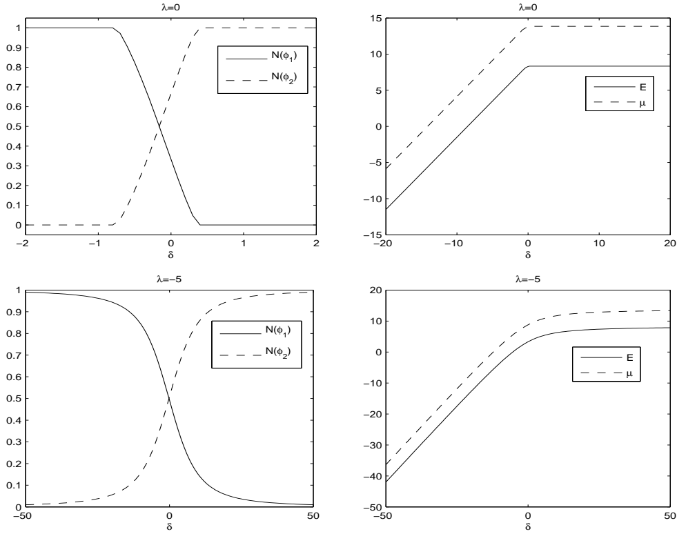
Figure 5: Mass of each component N(\phi_j) = \|\phi_j\|^2 ( j = 1, 2 ), energy E := E(\Phi_g) and chemical potential \mu := \mu(\Phi_g) of the ground states in Example 1 when \beta = 100 and \lambda = 0, -5 for different \delta .
