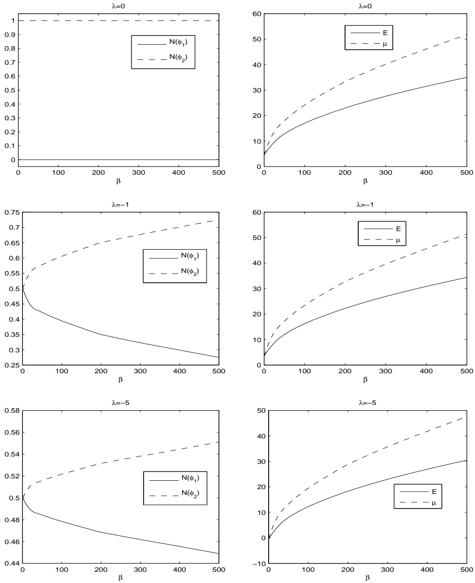
Figure 8: Mass of each component N(\phi_j) = \|\phi_j\|^2 ( j = 1, 2 ), energy E := E(\Phi_g) and chemical potential \mu := \mu(\Phi_g) of the ground states in Example 2 when \delta = 0 for different \lambda and \beta .
