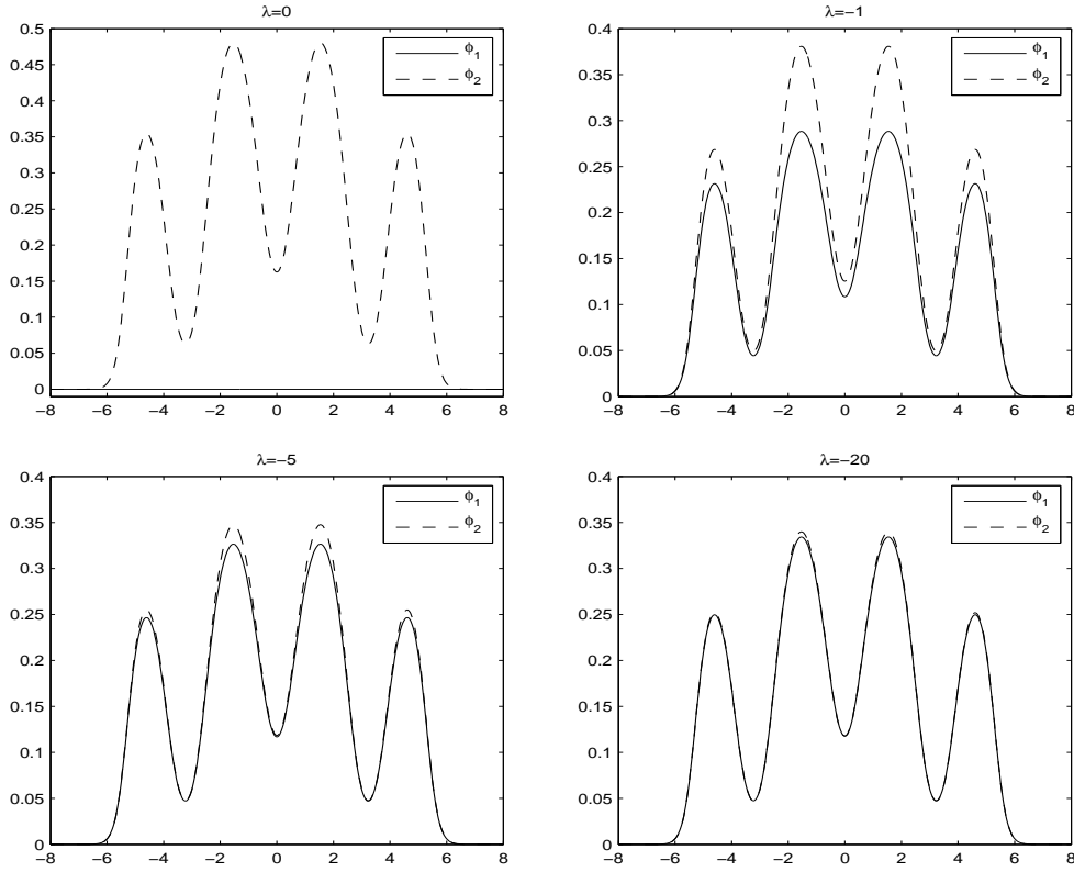
Figure 7: Ground states \Phi_g = (\phi_1, \phi_2)^T in Example 2 when \delta = 0 and \beta = 100 for different \lambda .
