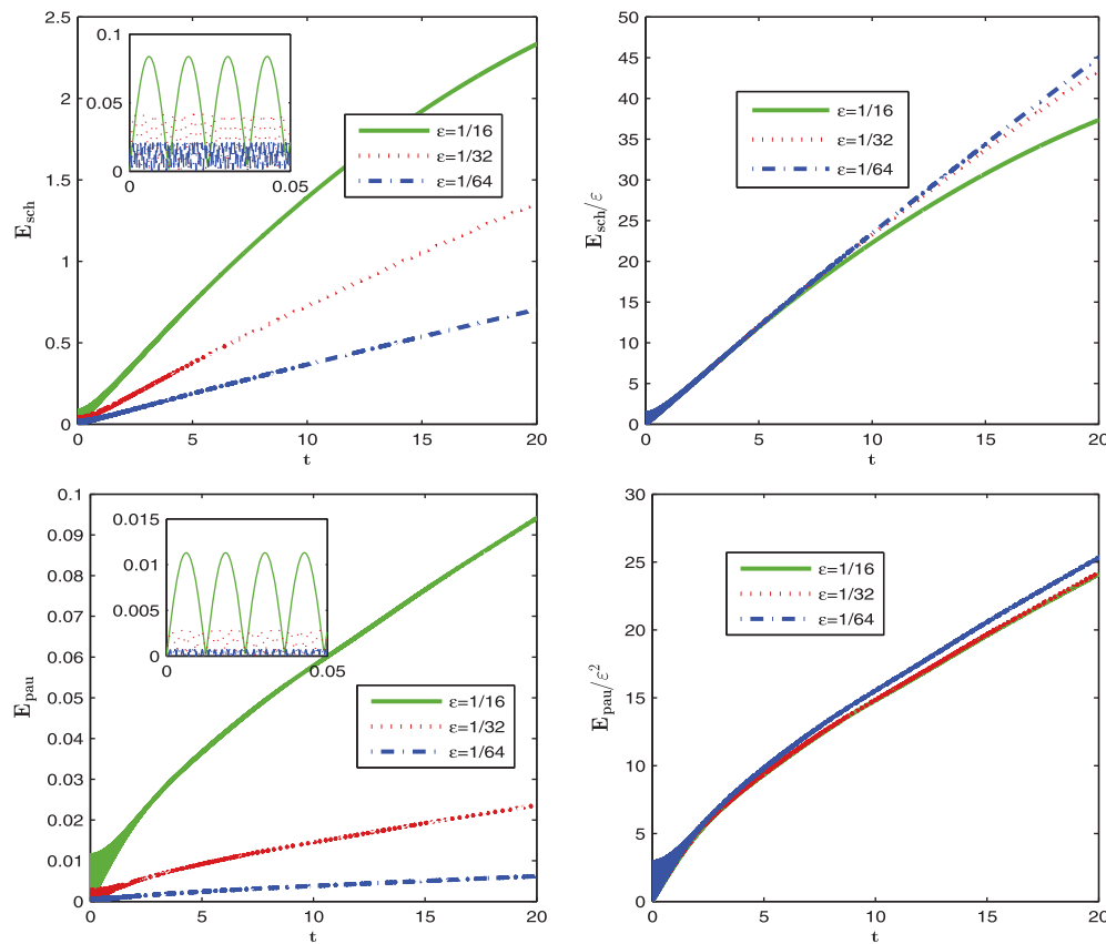
FIG. 1. Error functions E_{\text{sch}}(t) and E_{\text{pau}}(t) for different \varepsilon .
