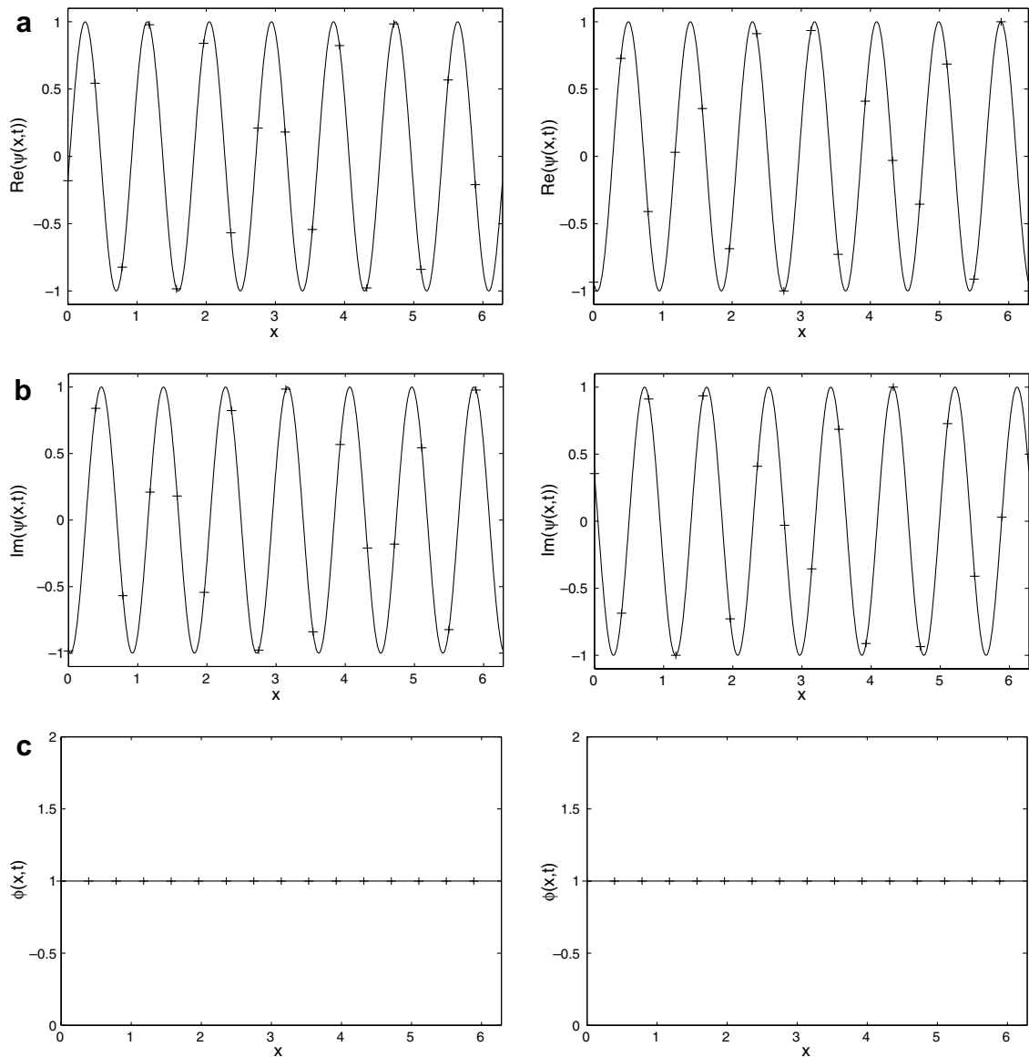
Fig. 3. Numerical solutions for the plane wave of KGS in Example 3 at time t = 2 (left column) and t = 4 (right column). ‘-’: exact solution given in (5.6), ‘+++’: numerical solution. (a): Real part of nucleon field \text{Re}(\psi(x, t)) ; (b): imaginary part of nucleon field \text{Im}(\psi(x, t)) ; and (c): meson field \phi .
