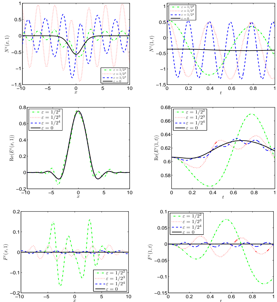
FIG. 1. The solutions of the ZS (1.1) for different \epsilon > 0 and the NLSE ( \epsilon = 0 ) as well as F^\epsilon defined in (2.1) with d = 1 . Here \text{Re}(c) denotes the real part of c .
