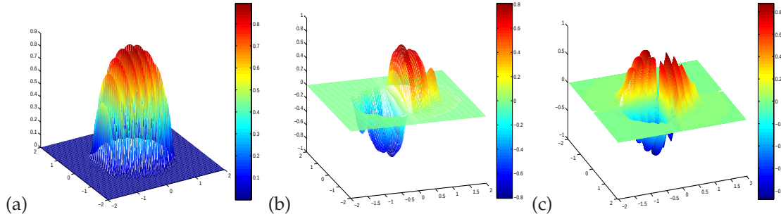
Figure 7: Surface plots for ground and asymmetric excited states of BEC with optical lattice potential in 2D with \varepsilon=0.025 . (a): Ground state; (b): asymmetric excited state in x -direction; (c): asymmetric excited state in both x - and y -directions.
