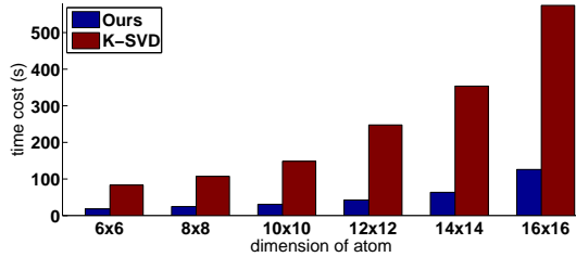
Figure 5. Overall running time of our method and the K-SVD denoising method with comparable PSNR values.
