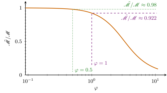
Fig. 1. Effect of pixel size on the reconstructed overall degree of coherence if pixel values were interpreted as point samples of the intensity. The horizontal axis gives the ratio ( \varphi ) of the pixel size to the standard deviation of the Gaussian intensity profile, and the vertical axis gives the ratio of the reconstructed overall degree of coherence ( \tilde{\mathcal{M}} ) to the true overall degree of coherence ( \mathcal{M} ) assuming noiseless measurements.
