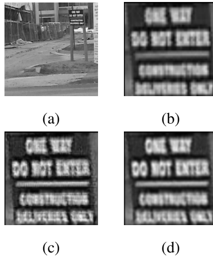
Fig. 12. (a) The key frame in the video. (b) The reconstruction from the interpolation. (c) The reconstruction from Irani's method using affine flow. (d) The reconstructed image from the wavelet method with de-noising using affine flow.
