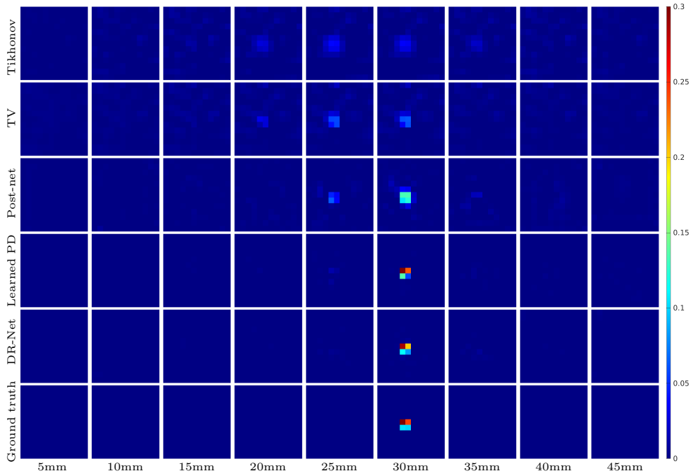
FIGURE 5. Reconstructed scattering coefficients from simulated measurements with phantom of 10mm \times 10mm \times 5mm in depth of 30mm .
