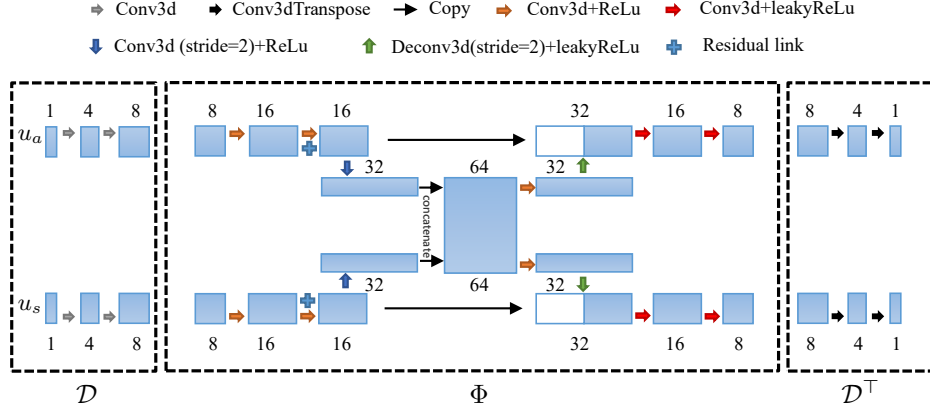
FIGURE 2. X-nets: architecture of components of DR-Net, including \mathcal{D}_\theta , \Phi_\theta and \mathcal{D}_\theta^\top . Note that the weights of \mathcal{D}_\theta and \mathcal{D}_\theta^\top can be shared with each other, or learned individually.
