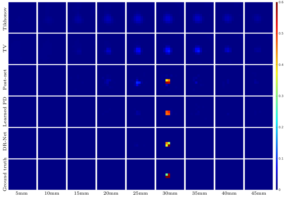
FIGURE 4. Reconstructed absorption coefficients from simulated measurements with phantom size of 10mm \times 10mm \times 5mm in depth of 30mm .
