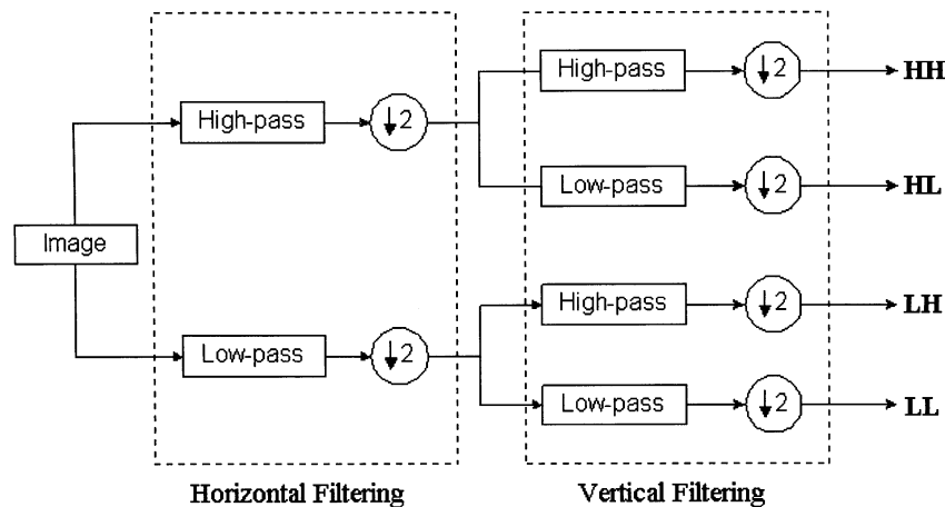
Fig. 1. Illustration of 2-D wavelet transform. 2-D DWT is generally carried out using a separable approach, by first calculating the 1-D DWT on the rows, and then the 1-D DWT on the columns.
