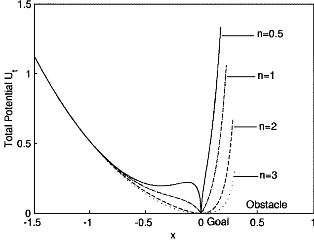
Fig. 6. Potential functions in a 1-D case.
