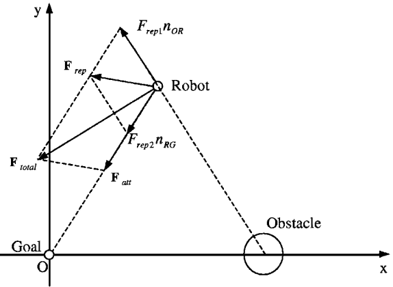
Fig. 5. Repulsive force derived by the new potential function.
