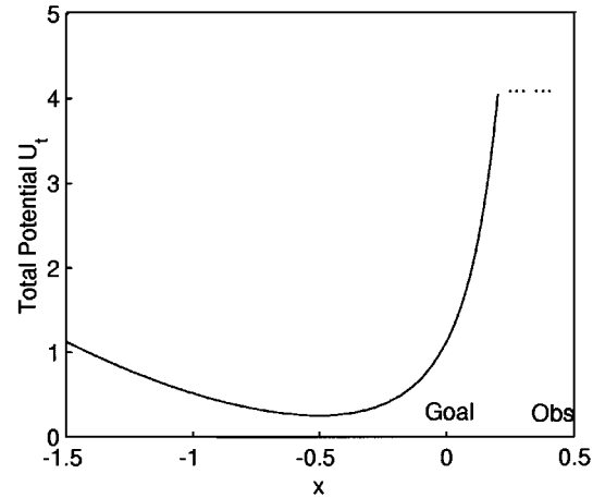
Fig. 2. Total potential function in a 1-D case.
