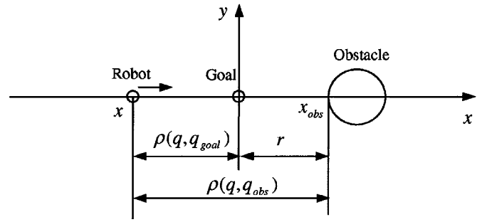
Fig. 1. Locations of the robot, goal, and obstacle in a 1-D case.
