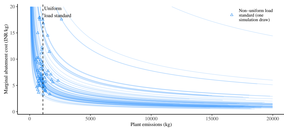
FIGURE VII Marginal Abatement Cost Curves for Treatment Plants
