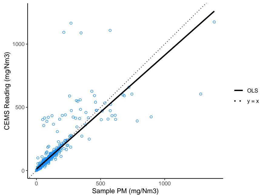
Figure F4. Simultaneous CEMS and Sampling Comparison
