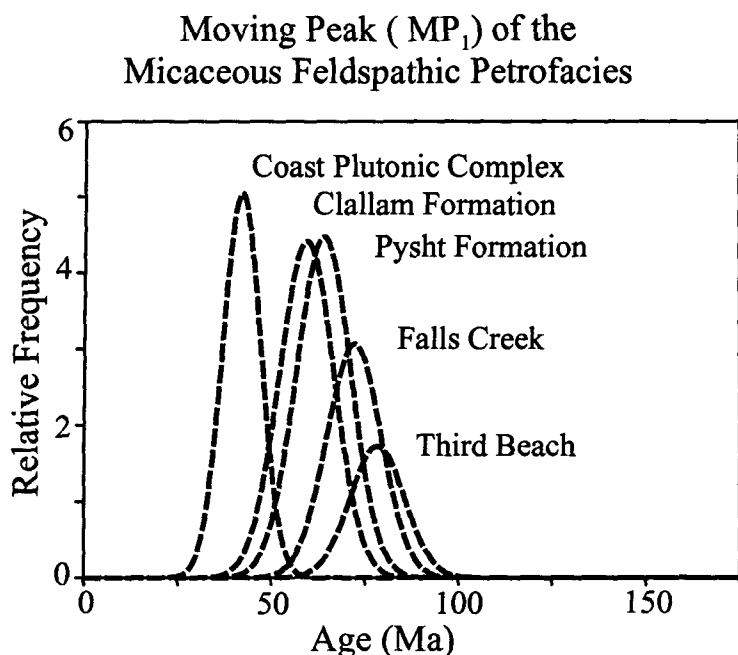
Figure 10. Plot of the age progression of the principal moving peaks in the micaceous feldspathic petrofacies and the presumed correlative peak in the modern Coast Ranges of British Columbia. Individual peaks are shown by their Gaussian distribution, and the height of the Gaussian is proportional to the percentage of zircon in each population.
