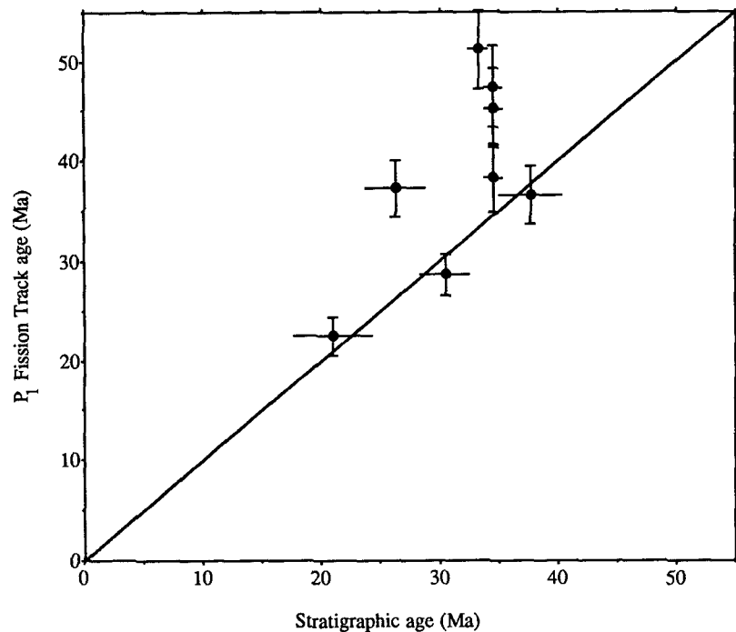
Figure 6. The relationship between the \chi^2 age and the P_1 age (both the youngest peaks) against stratigraphic age. Note that unlike other FT studies in the Pacific Northwest, most of these samples appear to lack a peak close to the depositional ages of the unit (diagonal line). The absence of a young peak is probably due to the lack of contemporaneous volcanics in the source region.
