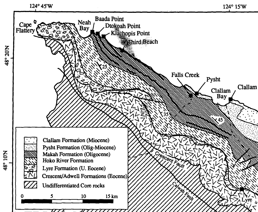
Figure 2. Geologic map (modified from Tabor and Cady, 1978b) of sample localities for the northwestern Olympic Peninsula. See Appendix for map coordinates and outcrop descriptions of each sample.
