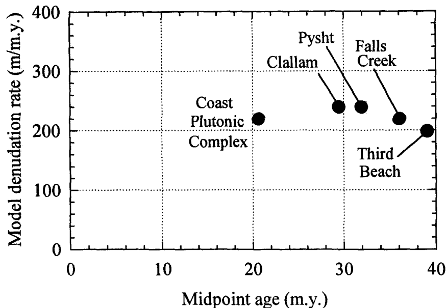
Figure 11. Model denudation rate through time as calculated for the principal peaks seen in the Clallam and Pysht Formations and the inferred correlative peaks in the Falls Creek unit and the Third Beach Member of the Makah Formation. Age plotted is the midpoint between the depositional age and the peak age (Brandon and Vance, 1993; see text for discussion and assumptions).
