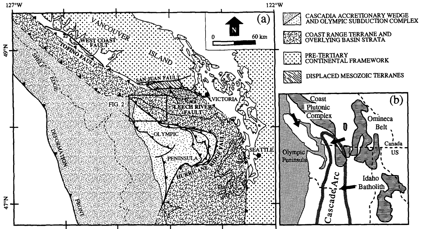
Figure 1. (a) Geologic map of the Pacific Northwest and the tectonic setting of the Olympic Mountains (modified from Clowes and others, 1987) showing the location of the study area (Fig. 2). Structurally above the Olympic Subduction Complex (OSC), which is the accretionary complex, is a sequence of Eocene basalts (Coast Range terrane) with an overlying sequence of Eocene and younger strata of the Tofino basin from the northwestern Olympic Mountains north along the west coast of Vancouver Island. On the northwestern part of the Olympic Peninsula, Eocene to lower Miocene strata of the Tofino basin are exposed in a north-dipping sequence. (b) The inset (modified from Brandon and Vance, 1992) shows the Cascade arc in southern British Columbia, Washington, and Oregon, as well as the distribution of the principal metaplutonic source regions in the Pacific Northwest. These source regions include the rapidly cooled plutonic and metamorphic rocks of the Idaho batholith and the Omineca Belt east of the Cascade arc, and the Coast Plutonic Complex, which is mainly north of the arc. Arrows represent the principal sediment paths for detritus that has accumulated in the area of the Olympic Mountains.
