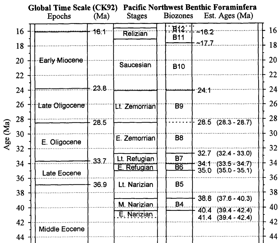
Figure 4. Correlation of the Pacific Northwest benthic foraminifera biozones (Rau, 1981; Armentrout, 1981; Prothero and Armentrout, 1985) to the time scale of Cande and Kent (1992). For this paper, we use the Pacific Northwest stages of Rau (1981; his Fig. 11) as correlated to the global time scale by Armentrout (1981), Armentrout and others (1983), and Prothero and Armentrout (1985). Cande and Kent (1992) is used for global correlation of epochs and magnetic chrons. All isotopic ages are relative to modern constants (see Harland and others, 1990), and all uncertainties are cited at the 95% confidence level (approximately \pm 2 standard error).
