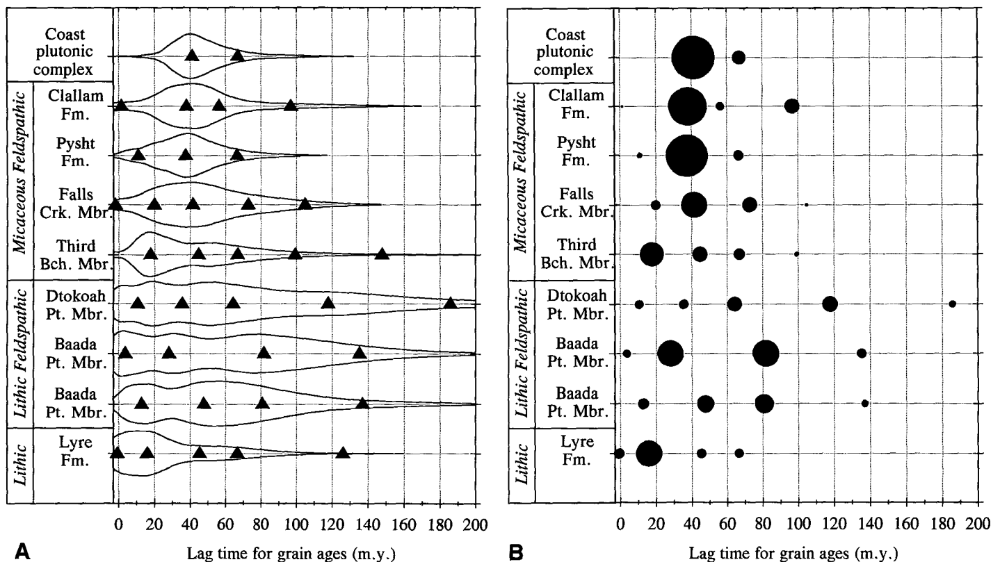
Figure 8. Summary of zircon FT data from all units studied and the zircon FT data from the Coast Plutonic Complex (Parrish, 1983; see Fig. 5) showing (A) lag time for individual peaks as well as the density plot, and (B) lag time for individual peaks and the proportion of grains in each peak. We interpret the progressive reduction in age of the peaks in the micaceous feldspathic petrofacies (from the Third Beach Member of the Makah Formation to the Clallam Formation) to represent the erosional unroofing and progressive cooling of a single plutonic source terrain.
