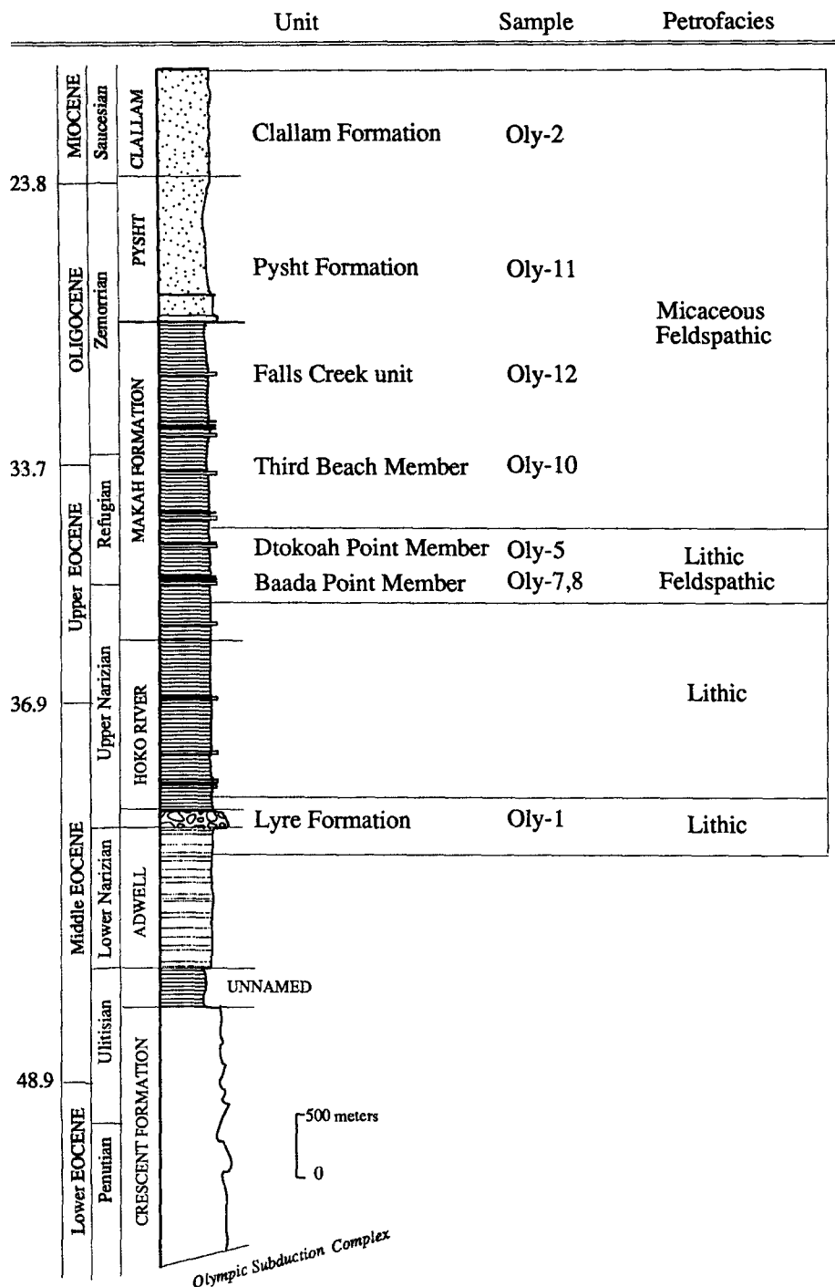
Figure 3. Stratigraphic column of the Tertiary sequence on the northwestern part of the Olympic Peninsula (modified from Muller and others, 1983) showing sample numbers with locations. Informal petrofacies designations, shown to the right, are discussed fully in the text. Strata of the Hoko River, Makah, and Pysht Formations comprise the Twin Rivers Group. Our estimate of the age of individual samples (Table 2) and stratigraphic units is shown to the left (Fig. 4, Table 2).
