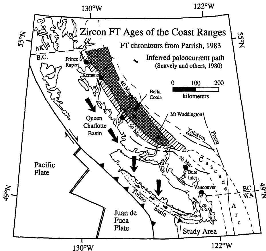
Figure 12. Zircon fission-track ages and plate tectonic setting of the Coast Plutonic Complex (CPC; modified from Parrish, 1983) and sediment transport direction in the upper Eocene to Oligocene strata of the Tofino basin (modified from Snively and others, 1980). Parrish calculates that the main axis of the Coast Plutonic Complex experienced a maximum of ~5–9 km of total denudation since 40 Ma, although part of this denudation (~2.0–3.5 km) has occurred since the late Miocene. The heavy solid arrows represent the probable path of sediment that fed the Tofino basin.
