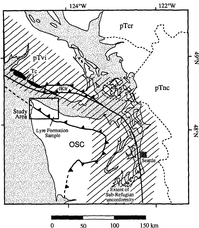
Figure 9. Generalized map of the Pacific Northwest showing our estimate of the limit of the sub-Refugian unconformity (diagonal ruled area) in this area. Stratigraphic sections in this diagonally ruled area have a prominent unconformity where Refugian and younger strata rest on either the Coast Range terrane or pre-Tertiary rocks (pTvi = pre-Tertiary rocks of Vancouver Island; pTnc = pre-Tertiary rocks of the North Cascades and the San Juan Islands; pTcr = pre-Tertiary rocks of the Coast Plutonic Complex; JKlr = Leech River Complex). Tc is the Carmanah Formation, which rests unconformably above the pre-Tertiary rocks of Vancouver Island, but also blankets the San Juan fault. The limits of the sub-Refugian unconformity is bounded by those areas where sub-Refugian Eocene sediments are preserved, indicating little or no erosion at the level of the unconformity.
