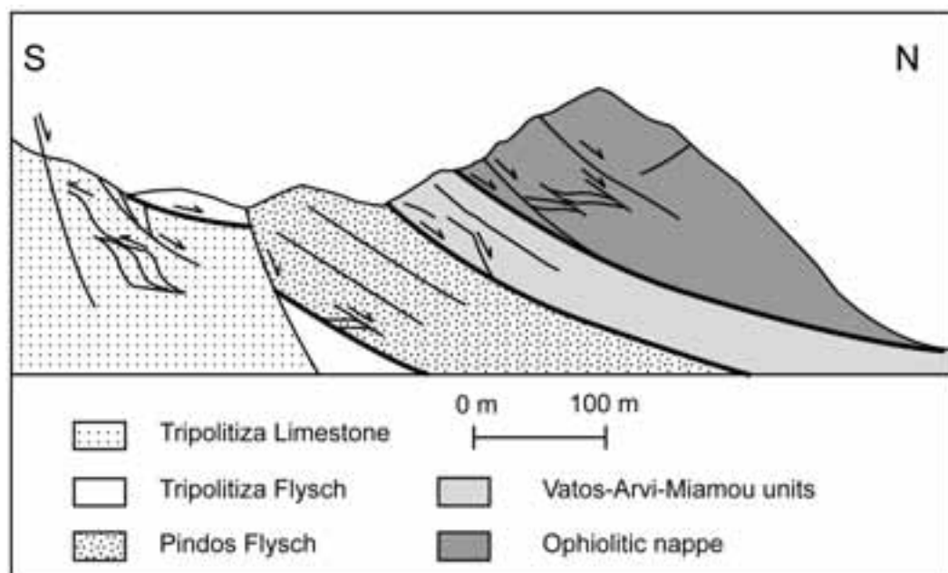
Figure 10 - Schematic cross-section illustrating the structure of the upper-plate units in the area of the village of Gonia (after Fassoulas et al., 1994).
