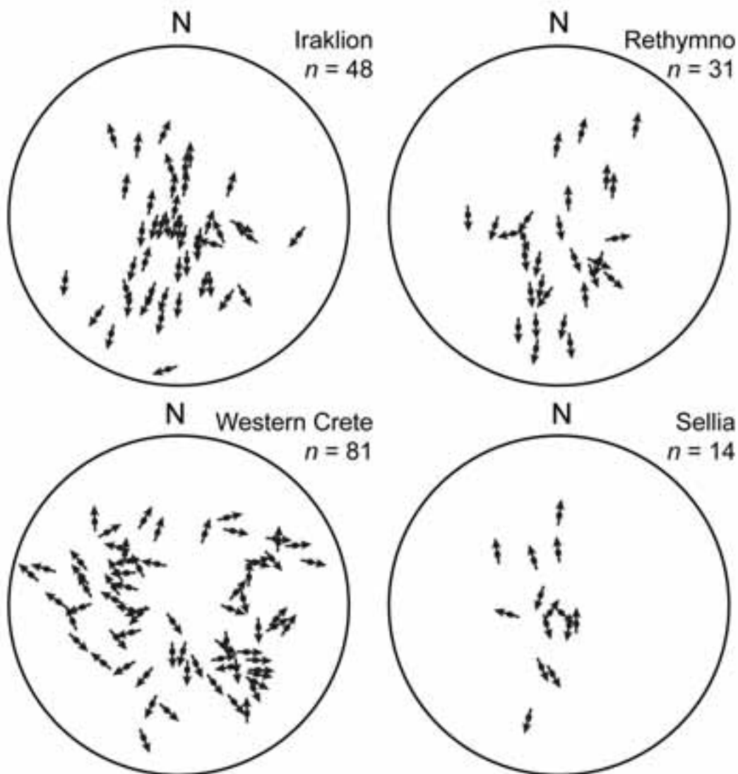
Figure 15 - Lower hemisphere stereonet projections showing slip-linear data for brittle fault zones within the Phyllite-Quartzite nappe in various areas in western and central Crete. Each square represents the pole to an individual fault plane. The arrow represents the direction of motion of the footwall block relative to a fixed hanging wall block. (Arrows pointing away from the center of stereonet indicate normal-sense slip.) Fault planes show a variety of orientations and nearly all record normal-sense slip.
