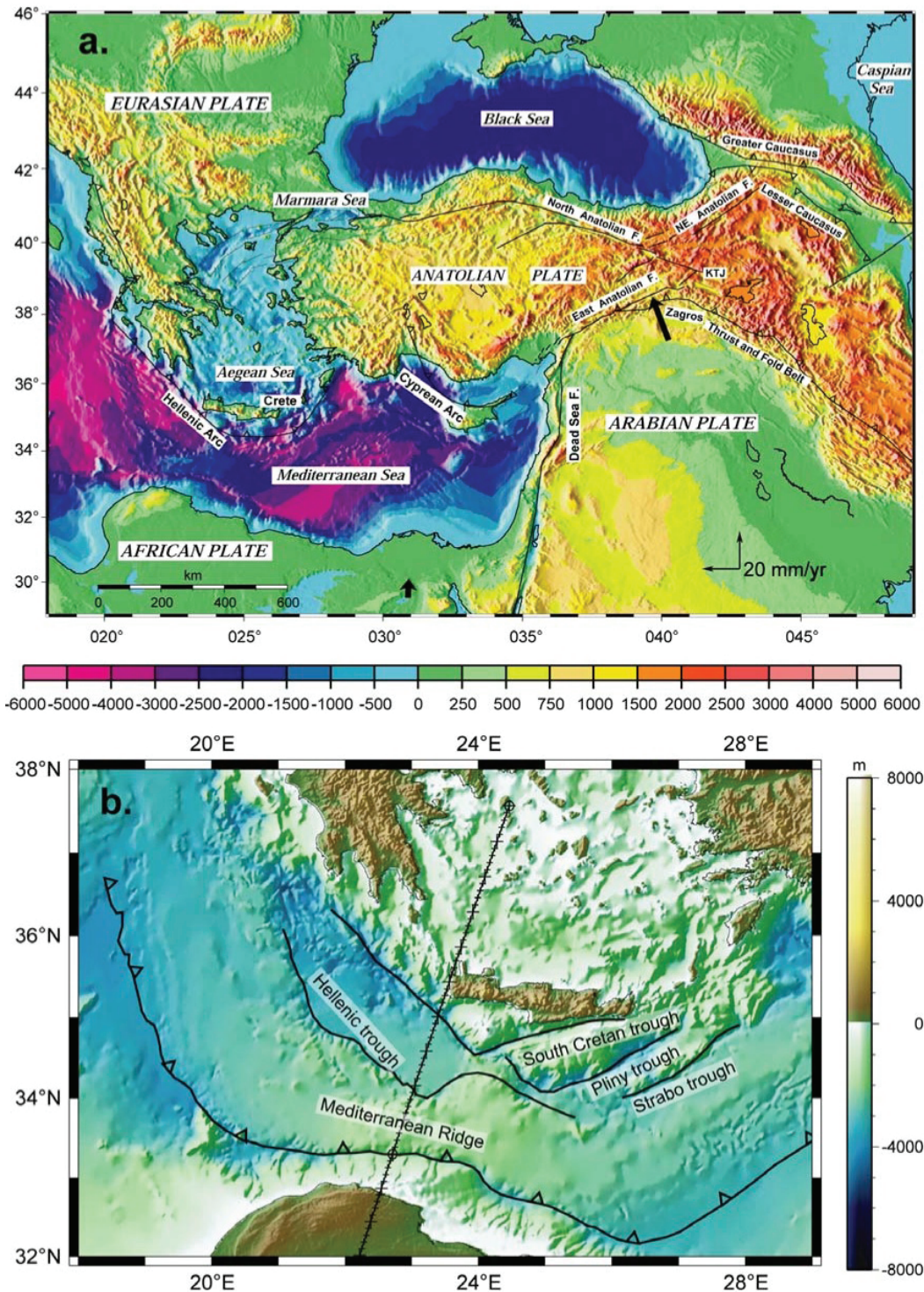
Figure 1 - a) Simplified tectonic map of the eastern Mediterranean region, from McCluskey et al. (2000). Structures are superimposed on topography and bathymetry. Heavy arrows show NUVEL-1A plate motions relative to Eurasia. KTJ – Karliova triple junction. b) Topography and bathymetry of the eastern Mediterranean. Line shows location of cross-section in Figure 2.
