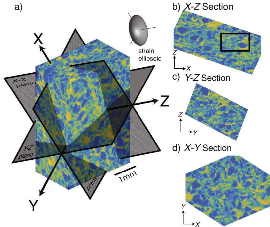
Fig. 13. Tomogram for deformed sandstone (sample 92810-3 from the Olympic subduction complex). (a) 3D rendering showing principal strain axes and sections as determined using the ACF method. (b–d) Slices through the tomogram along principal strain sections. See Table 2 for results. The black box in panel (b) outlines the region shown in Fig. 14.
