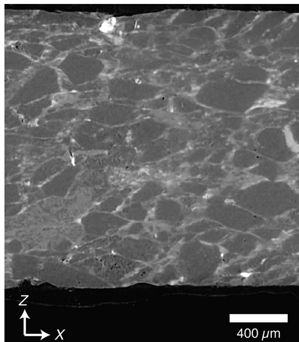
Fig. 1. X-ray tomography image of an X–Z section through a sandstone deformed by pressure solution (sample 92810-3 from the Olympic subduction complex in NW Washington State). A deformation fabric is indicated by detrital grains (dark gray), which are separated by anastomosing cleavage surfaces (long, thin light-gray features, approximately parallel to the X direction) and by directed overgrowths (thicker light-gray features, oriented in the X direction). The cleavages have accommodated shortening in the Z direction, and the overgrowths, extension in the X direction.
