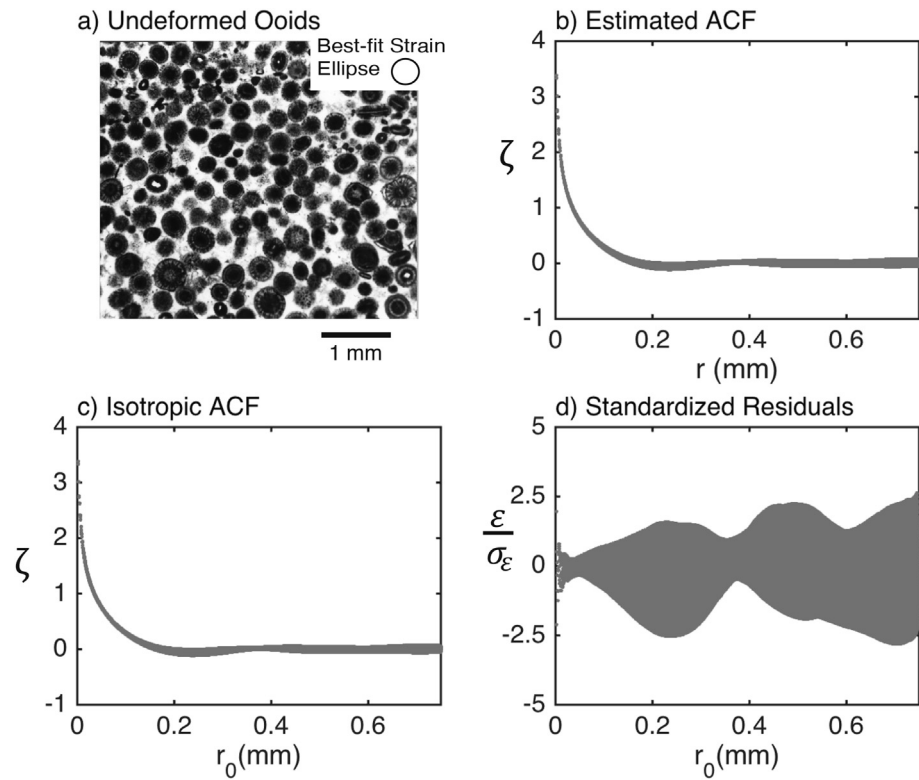
Fig. 10. Use of ACF method to estimate strain for (a) 2D photomicrograph of undeformed ooids from the Jurassic Stump formation in Wyoming (Crespi, 1986). See caption in Fig. 9 for details of (b–d), and Table 1 for results.
