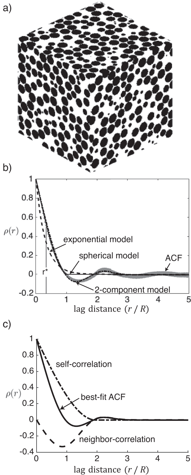
Fig. 7. Comparison of ACF model functions. (a) A 3D synthetic aggregate composed of non-overlapping identical spheres. (b) The ACF for the synthetic aggregate (gray line) and best-fit solutions using the exponential model (dash line), the spherical model (solid line), and the 2-component model (dash-dot line). The “half-height” lag is shown by r^* . (c) The best-fit 2-component model (solid line) and the self-correlation (dash-dot line) and neighbor-correlation (dash line) components for that fit.
