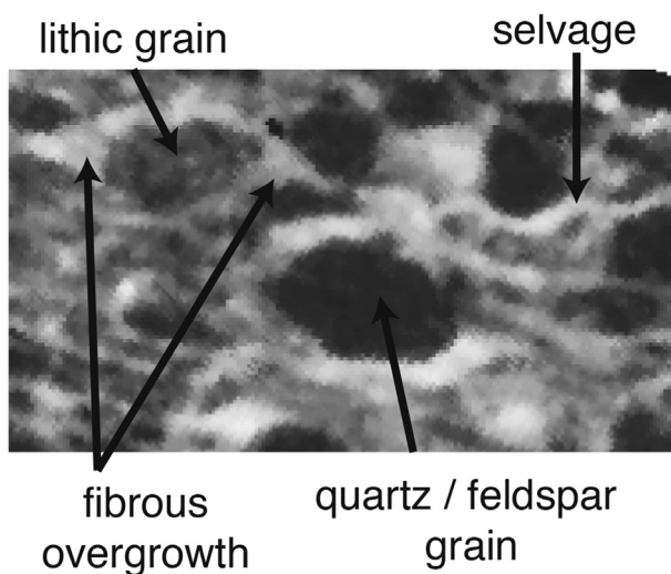
Fig. 14. Pressure-solution fabric elements in X-Z slice of sample 92810-3 tomogram. Arrows indicate quartz/feldspar and lithic grains, fibrous overgrowths, and selvages. The magnified view is outlined by the black box in Fig. 13b.
