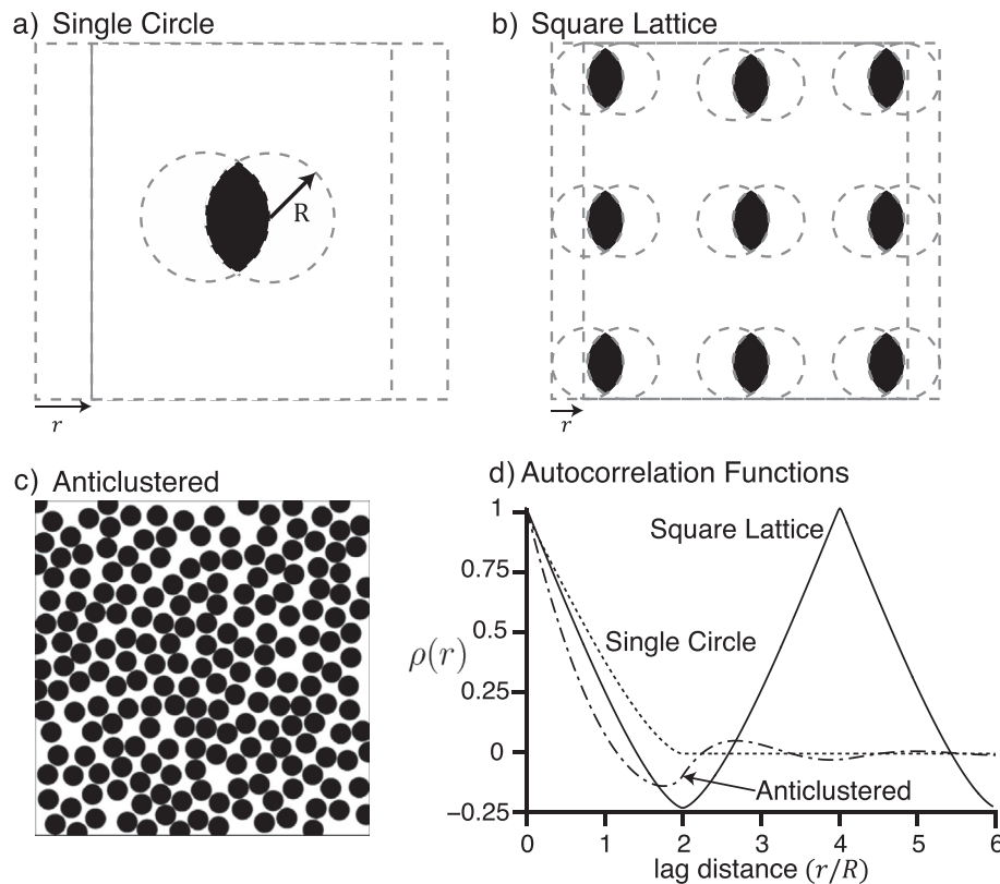
Fig. 4. The autocorrelation function for three examples: (a) a single circle, (b) a square lattice of circles, and (c) an anticlustered distribution of circles. (d) The autocorrelation function \rho(r) for these examples is related to the change in the overlapping area of the circles, which is set to 1 when the lag r = 0 , and decreases as the lag increases to R , the radius of the circles.
