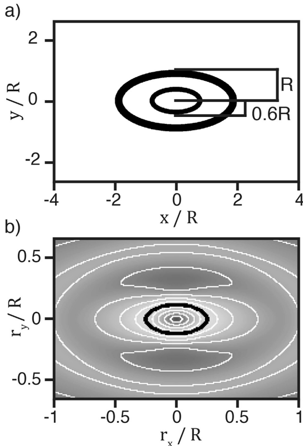
Fig. 12. The effect of internal particle structure on the ACF. (a) A test object composed of concentric rings with the same aspect ratio. (b) The ACF contours are not everywhere elliptical, but instead have “hot-dog” shapes at intermediate lags. The black line is r .
