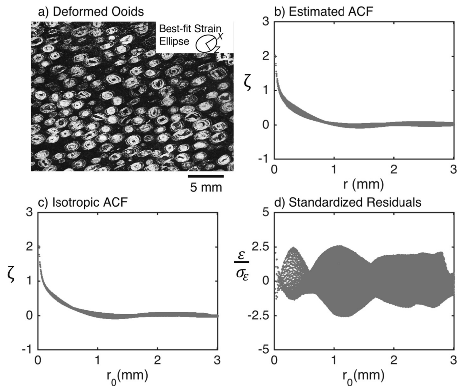
Fig. 11. Use of ACF method to estimate strain for (a) 2D photomicrograph of deformed ooids (figure 7.7 in Ramsay and Huber, 1983). See caption in Fig. 9 for details of (b–d), and Table 1 for results.
