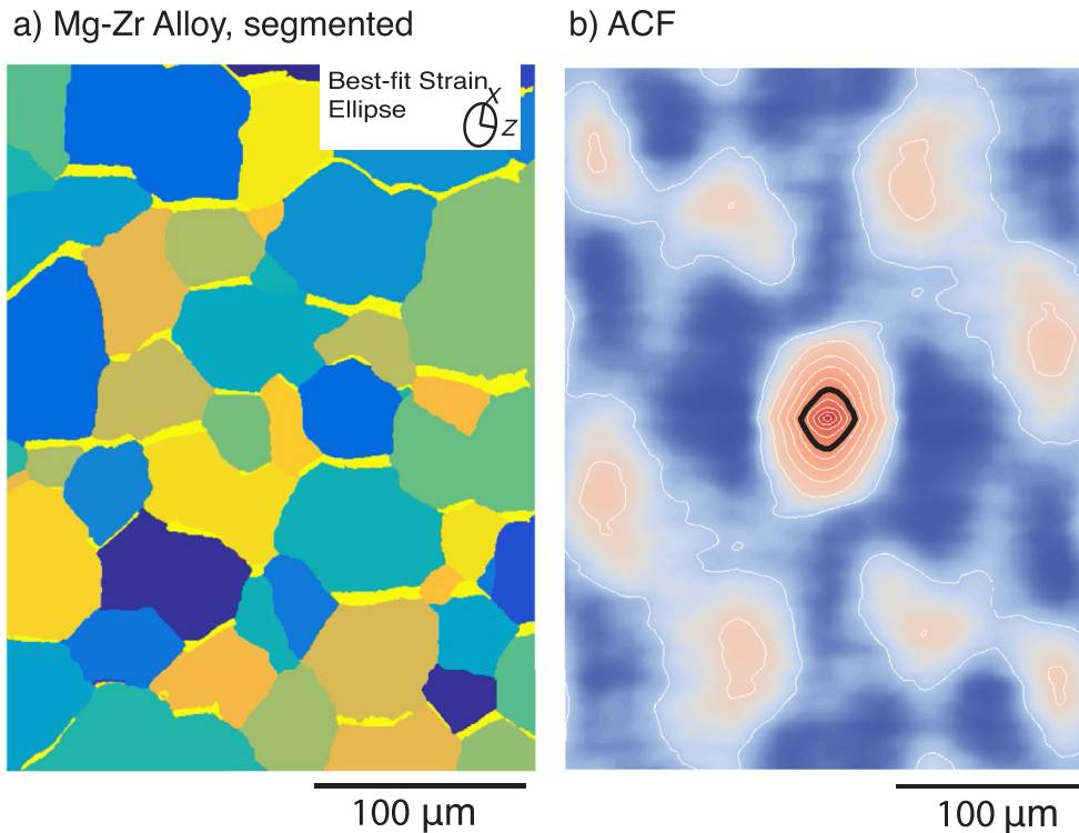
Fig. 16. Segmentation of the “grains” in the Mg–Zr alloy dramatically changes the best-fit strain results. (a) The “grains” are manually segmented and assigned uniform grayscale values. (b) The ACF suggests the segmented grains are elongated in the vertical direction. Black line marks the r_0^2 contour. See Table 1 for results.
