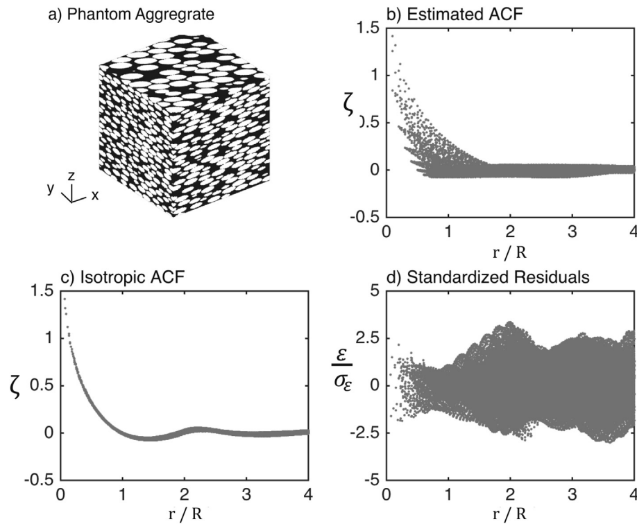
Fig. 9. Synthetic example (phantom) used to test the ACF method for estimating 3D strain. (a) A 3D rendering of the phantom, which was constructed from identical non-overlapping spheres and then deformed homogeneously. (b) Observed ACF in the deformed coordinate frame with lag normalized to the radius R of the undeformed spheres. (c) Isotropic ACF, determined by removing estimated strain. (d) Standardized residuals for the best-fit isotropic ACF as a function of lag.
