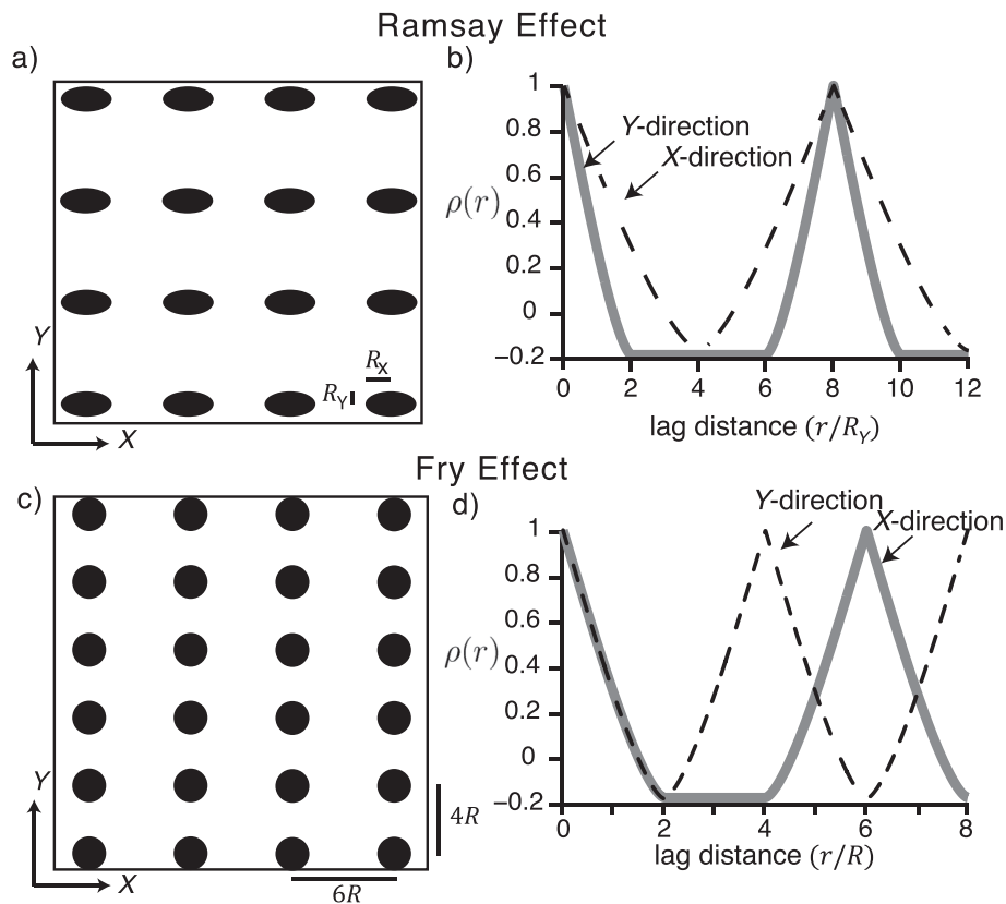
Fig. 5. The Ramsay and Fry effects in the ACF. (a, b) At short lags, where r/R < 1 , the ACF represents the correlation of features with themselves, and thus the ACF is sensitive to the anisotropy of features. The anisotropy in this range is similar to that measured by the Ramsay method, which is focused on the distortion of features. (c, d) At long lags, where r/R > 1 , the ACF is sensitive to the anisotropic distribution of features with respect to each other. This anisotropy is similar to that measured by the Fry method, which focuses on the distribution of nearest neighbors.
