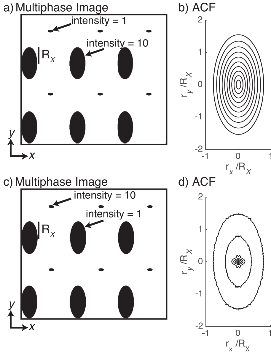
Fig. 6. Two examples showing how the ACF is affected by the contrast in intensity between phases. The ACFs for these examples are shown as contours of \rho in terms of x and y components of the lag vector and a contour interval of 0.1. (a) For the first example, the gray ellipses are small and have little contrast with the surrounding white phase, so (b) the ACF contours everywhere mimic the anisotropy of the larger black ellipses. (c) For the second example, the black ellipses are small, but have high contrast with respect to the other two phases. (d) As a result, the ACF contours have the same elliptical shape as the black phase at short lags ( r/R_x \sim 0.1 ), but take on the elliptical shape of the gray phase at long lags ( r/R_x > \sim 0.3 ).
