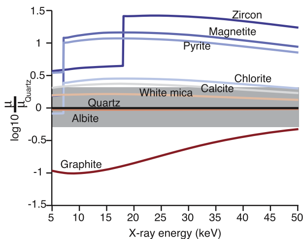
Fig. 2. X-ray attenuation coefficients for various geologic materials (Chantler et al., 2005), as normalized by the coefficient for quartz. The gray regions show a factor of two range for an attenuation coefficient relative to that for quartz. Minerals that lie outside that range are easily resolved relative to quartz in an X-ray tomogram.
