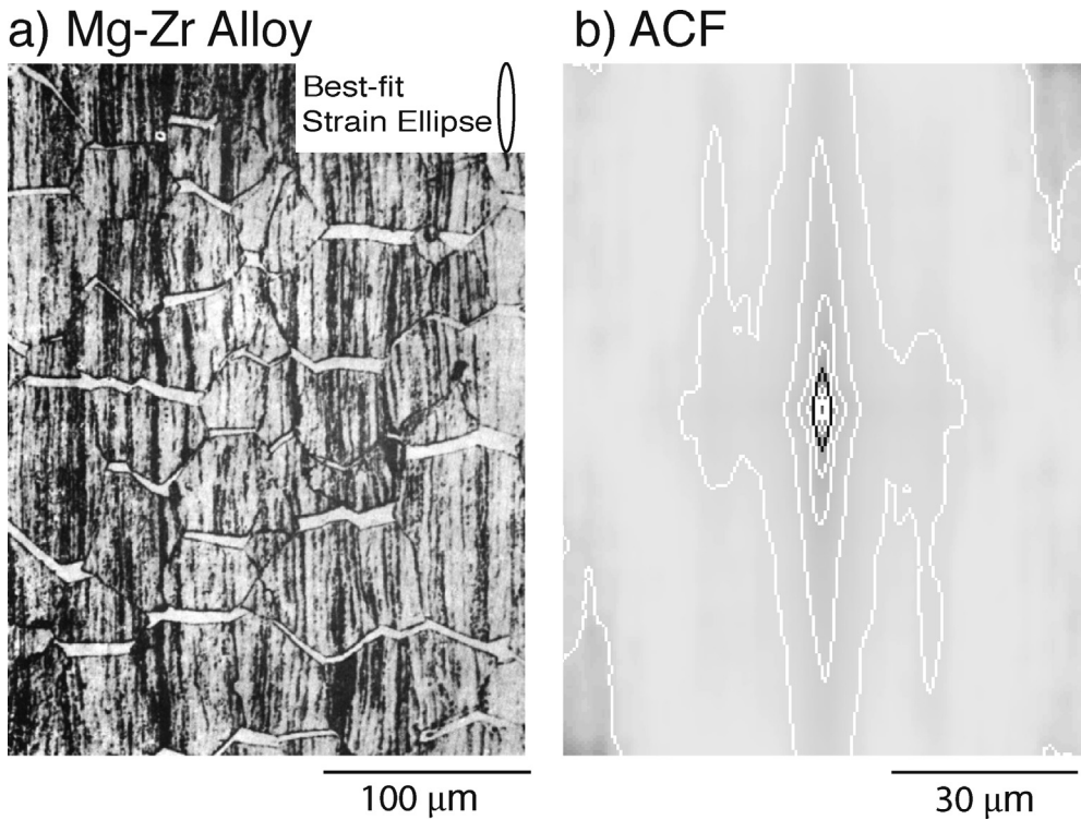
Fig. 15. A cautionary tale for using the ACF method. (a) Photomicrograph and (b) ACF of an Mg–Zr alloy that was initially formed by rolling, which produced the vertical laminar structure. The horizontal light gray zones in (a) are overgrowths that formed under high temperature conditions. During this deformation, the fabric was also broken into blocky domains by shear fractures. See Table 1 for results.
