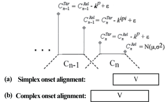
Figure 2: Summary of word simulation in the model. Consonant landmarks are generated from the release of the immediately prevocalic consonant. The alignment of the vowel is determined by the syllable parse (simplex or complex).
