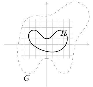
Figure 28.1.1: A square grid covering G .
