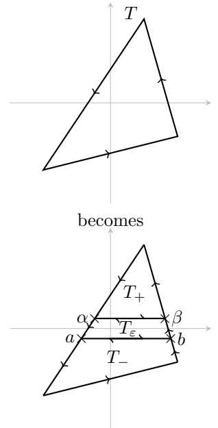
Figure 29.1.3: Partitioning a triangular path crossing the real axis.
