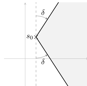
Figure 29.2.1: The sector in the setup.
