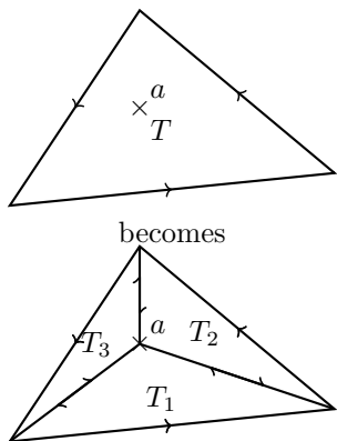
Figure 7.1.2: Dividing a triangular path T into three triangular paths T_1 , T_2 , and T_3 .
