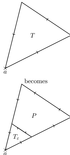
Figure 7.1.1: Decomposing a triangular path T into a smaller triangular path T_\varepsilon and a quadrilateral path P .
