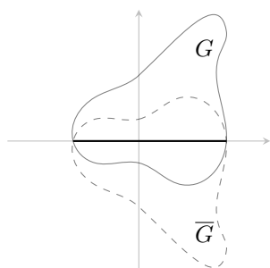
Figure 29.1.1: Two regions G and \bar{G} meeting on the real axis.
