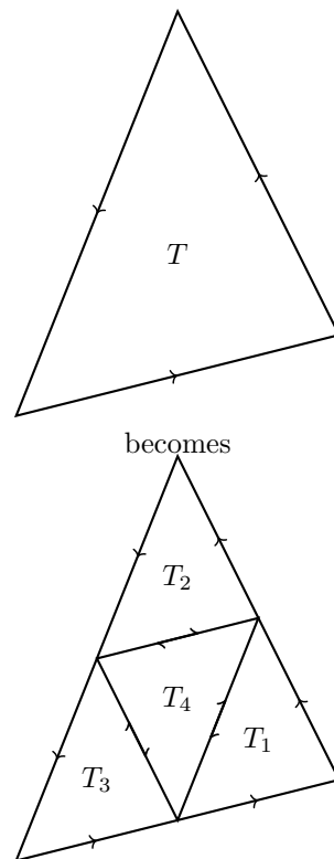
Figure 6.2.1: Decomposing a triangular path T into smaller triangular paths.
