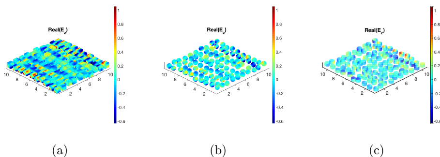
FIG. 13. Electric field component E_z in 10 \times 10 scatterer arrays with a TE incident wave in a half-space: (a) cubic scatterer with 27 collocation points in each, (b) spherical scatterer with 27 collocation points in each, and (c) cylindrical scatterer with 72 collocation points.
