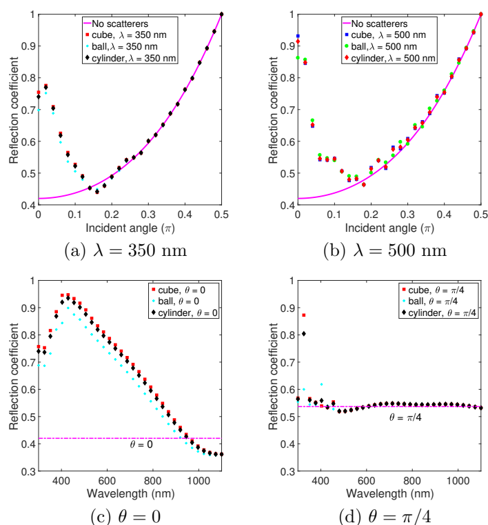
FIG. 14. Reflection coefficients calculated from the VIE for 3-D MMs in a half-space: (a) and (b) against incident angle and (c) and (d) against wavelength of a TE incident wave.
