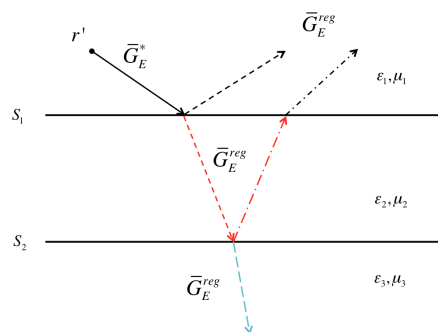
FIG. 3. Illustration of the layered Green's function. Interfaces S_1 and S_2 separate three layers of materials with dielectric constant \varepsilon_i and permittivity \mu_i ( i = 1, 2, 3 ). The overall layered Green's function is made of a primary, or singular, part and a regular part. Solid black lines represent the primary, or singular, part throughout all three layers. Dashed black lines are the regular part of the layered Green's function in the first layer, including the reflected part from S_1 and the transmitted part from the second layer. Red dashed lines are the regular part in the second layer, including the transmitted part from S_1 and the reflected part from S_2 . Finally, the blue dashed line represents the regular part in the third layer, which is the transmitted field from the second layer.
