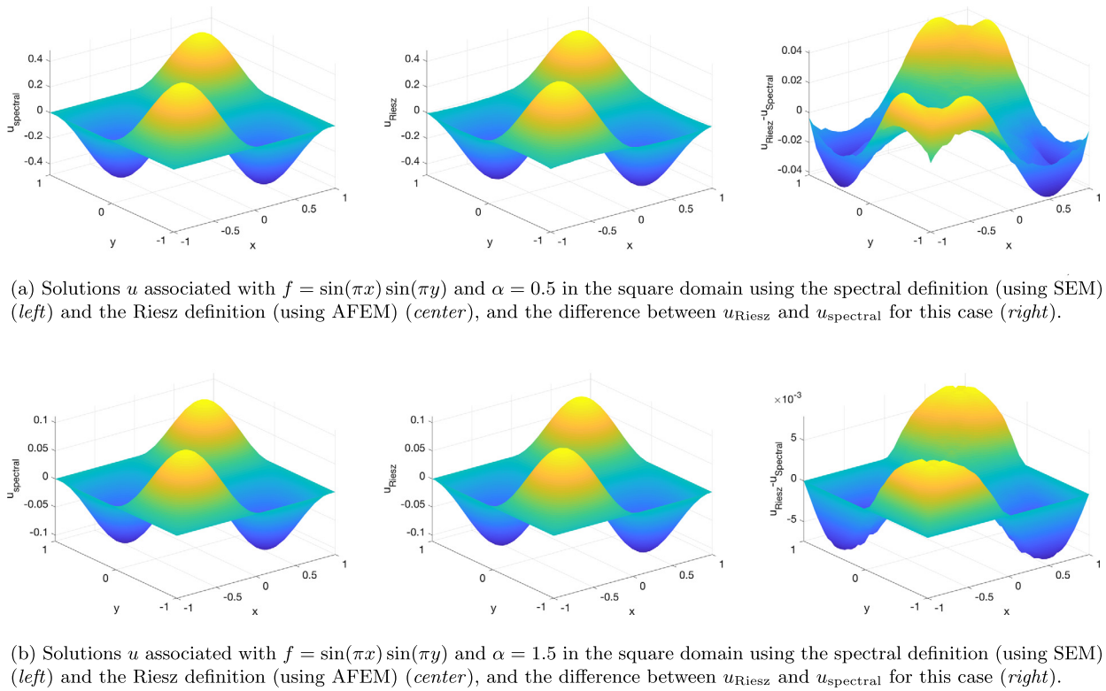
Fig. 16. Solutions and differences between u_{\text{Riesz}} and u_{\text{spectral}} on the square domain for \alpha = 0.5 and 1.5 .
