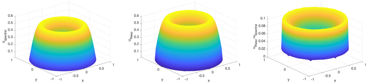
(a) Solutions u associated with f = \sin(\pi r^2) and \alpha = 0.5 in the disk domain using the spectral definition (using SEM) ( left ) and the Riesz definition (using AFEM) ( center ), and the difference between u_{Riesz} and u_{spectral} for this case ( right ).
