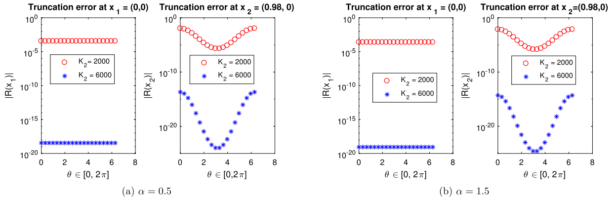
Fig. 6. Absolute values of truncation errors |R(x_i)| (69) for the modified GL formula (68) evaluated at the collocation points x_1 = (0, 0) and x_2 = (0.98, 0) . Two truncation parameters K_2 = 2000 and K_2 = 6000 are considered. Subplots (a) and (b) correspond to \alpha = 0.5 and \alpha = 1.5 , respectively.
