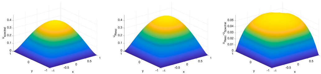
(b) Solutions u associated with f = 1 and \alpha = 1.5 in the square domain using the spectral definition (using SEM) (left) and the Riesz definition (using AFEM) (center), and the difference between u_{\text{Riesz}} and u_{\text{spectral}} for this case (right).
