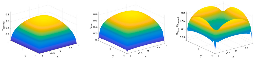
(a) Solutions u associated with f = 1 and \alpha = 0.5 in the square domain using the spectral definition (using SEM) (left) and the Riesz definition (using AFEM) (center), and the difference between u_{\text{Riesz}} and u_{\text{spectral}} for this case (right).
