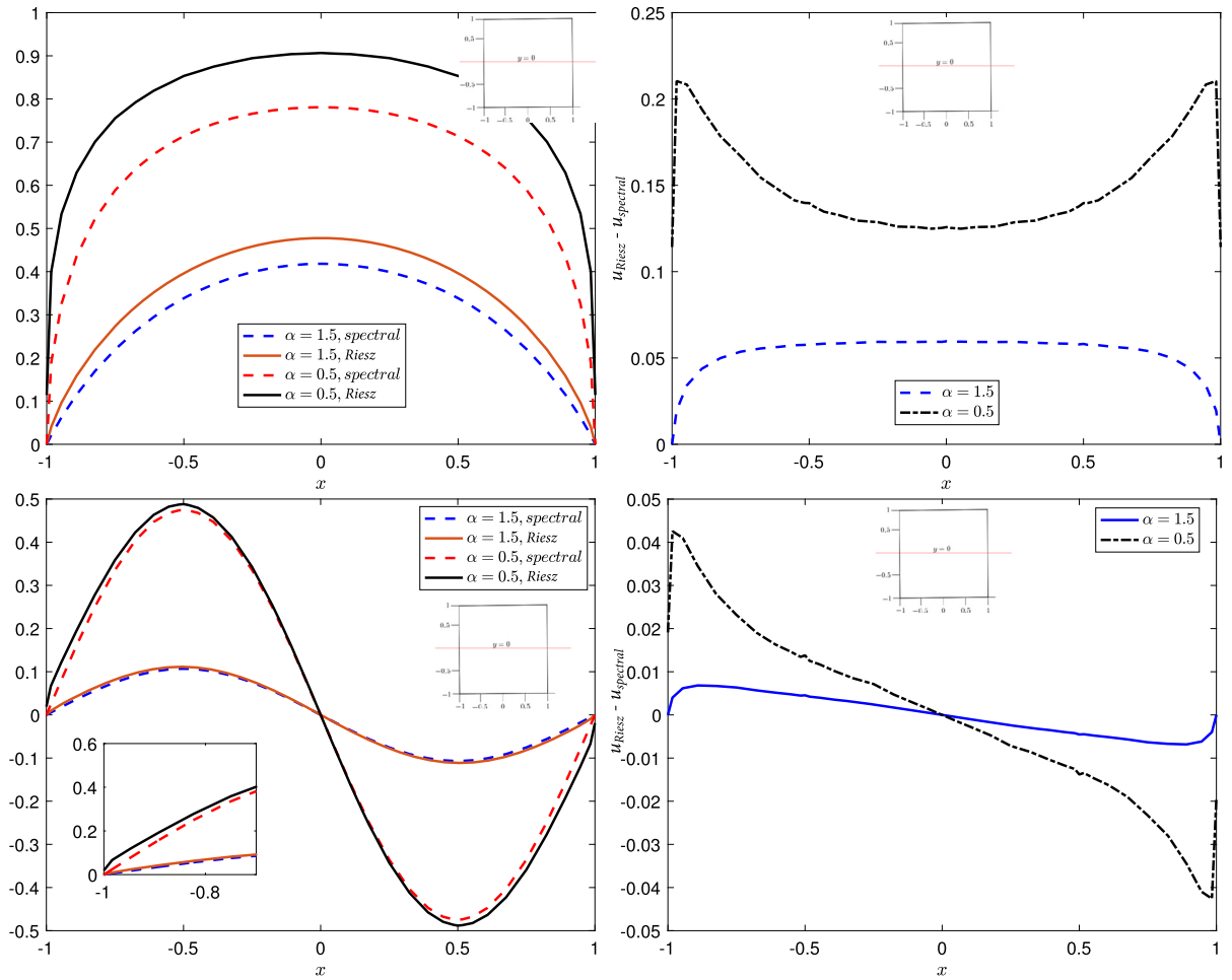
Fig. 17. Slices along the line y=0 in the square domain with both \alpha=0.5 and \alpha=1.5 . (top left) Plots of the solutions for the Riesz and spectral formulations with f=1 and (top right) plot of the differences u_{\text{Riesz}} - u_{\text{spectral}} along the line y=0 with f=1 . (bottom left) Plots of the solutions for the Riesz and spectral formulations with f=\sin(\pi x)\sin(\pi y) and (bottom right) plot of the differences u_{\text{Riesz}} - u_{\text{spectral}} along the line y=0 with f=\sin(\pi x)\sin(\pi y) . Some small wiggles that appear in the difference plots are due to the computation of the differences on two different meshes, even though the solutions are sufficiently converged and stable.
