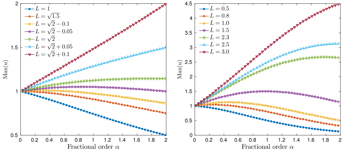
Fig. 2. Monotonicity study: (left) The maximum value of the numerical solutions for the spectral fractional Poisson equation (1) in the interval (-L, L) for \alpha \in (0, 2) with f(x) = 1 . (right) The maximum value of the numerical solutions for the Riesz fractional Poisson equation in the interval (-L, L) for \alpha \in (0, 2) with f = 1 .
