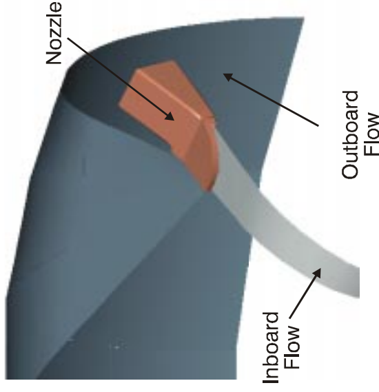
View of convective layer forming device - single nozzle
