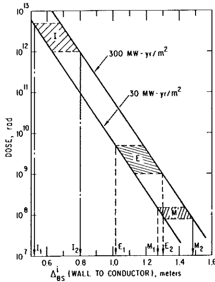
Fig. 6. Variation of Dose in TFC Insulators with \Delta_{BS}^i .
