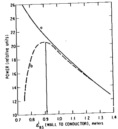
Fig. 3. Variation of (a) Gross Thermal Power; and (b) Gross Thermal Power Minus Refrigeration Power with \Delta_{BS}^i .
