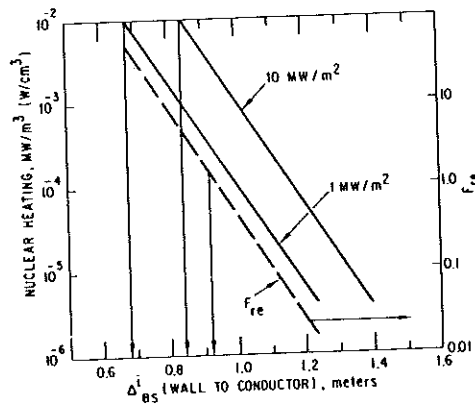
Fig. 2. Variation of the Maximum Heating and f_{re} in TFC with \Delta_{BS}^i .
