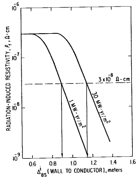
Fig. 5. Maximum Radiation-Induced Resistivity, \rho_r , as a function of \Delta_{BS}^i .
