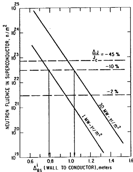
Fig. 4. Maximum Neutron Fluence in TFC Versus \Delta_{BS}^i .
