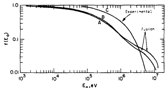
Fig. 20. The fraction, f(E_0) of the total neutron flux with neutron energies above E_0 as a function of E_0 for the three cases A, B and C shown in fig. 19.
