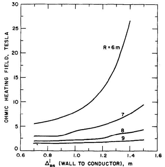
Fig. 8. Maximum ohmic heating field required in several size tokamaks as a function of inner blanket/shield thickness ( A = 3 , P_w = 3 \text{ MW/m}^2 , circular plasma).
