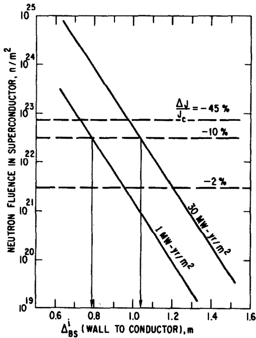
Fig. 9. Maximum neutron fluence is TF magnet as a function of inner blanket/shield thickness.
