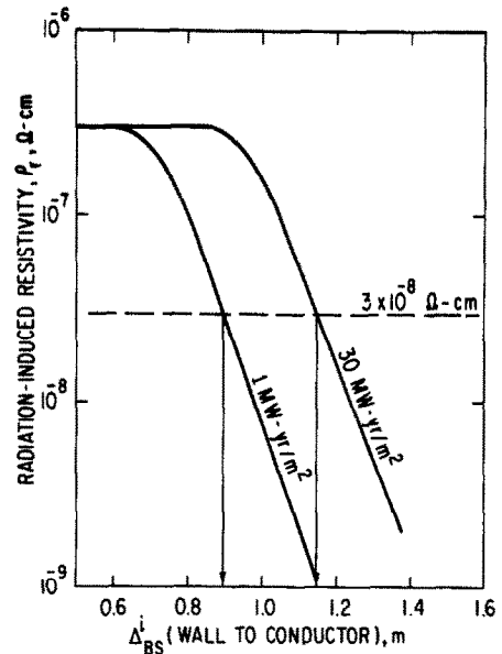
Fig. 10. Maximum radiation induced resistivity in copper stabilizer as a function of inner blanket/shield thickness.
