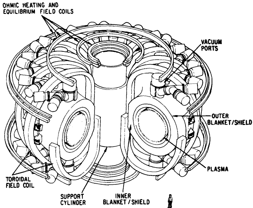
Fig. 1. Perspective view of a tokamak.
