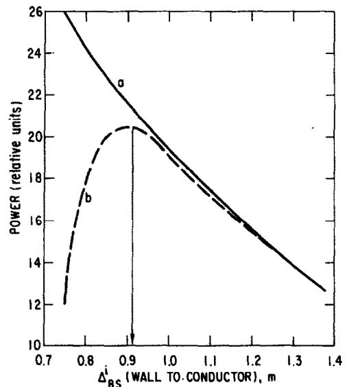
Fig. 5. Effect of inner blanket/shield thickness on (a) reactor gross electric power; and (b) reactor net electric power (= gross power – TF magnet refrigeration power).
