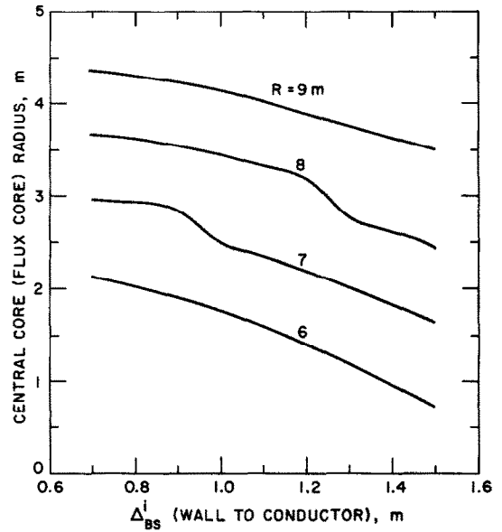
Fig. 7. Central core radius as a function of inner blanket/shield thickness for several size tokamaks ( A = 3 , P_w = 3 \text{ MW/m}^2 , circular plasma).
