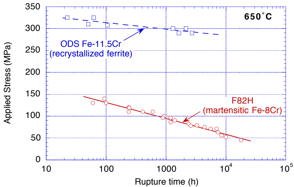
Fig. 8. Creep rupture strength of F82H martensitic steel and ODS ferritic steel [1,5,10,15].
