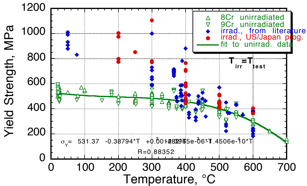
Fig. 3. Comparison of the yield strength of unirradiated and irradiated 8-9%Cr steels [6].
