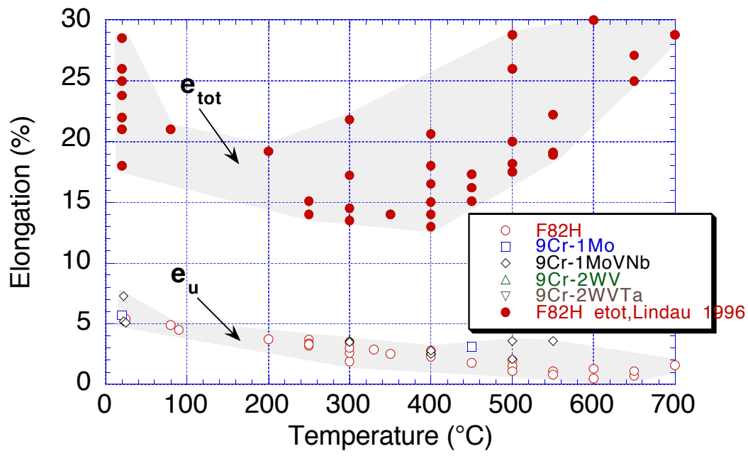
Fig. 4. Uniform and total elongation of unirradiated 8-9%Cr steels [1-3,6].
