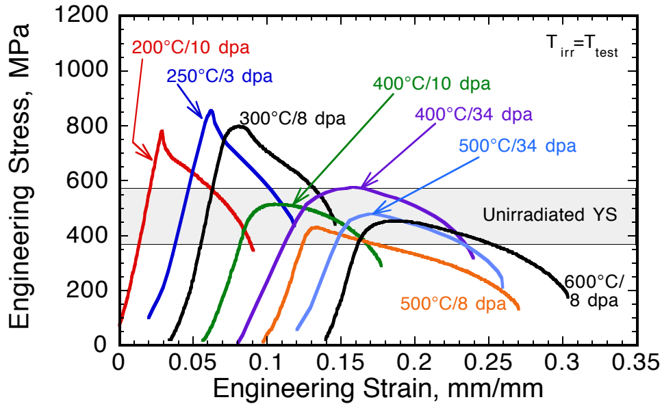
Fig. 7. Load vs. normalized crosshead displacement tensile curves for F82H irradiated to 3-34 dpa at 200-600°C [6,9,12].
