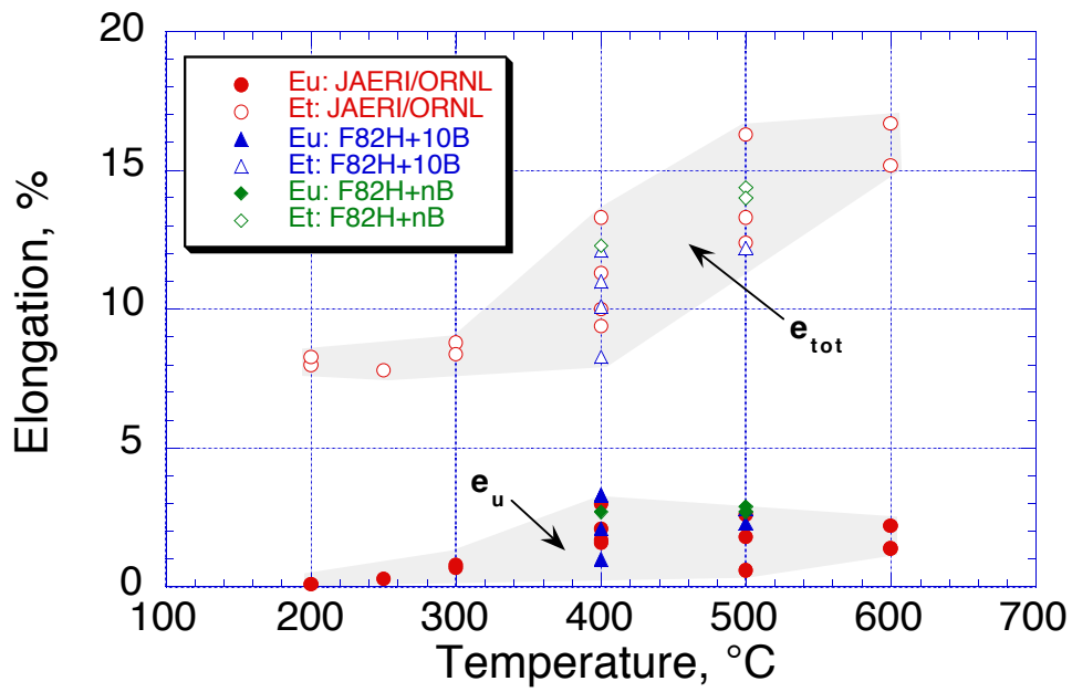
Fig. 5. Uniform and total elongation of irradiated 8-9%Cr steels [1-3,6]. The test temperature equals the irradiation temperature.
