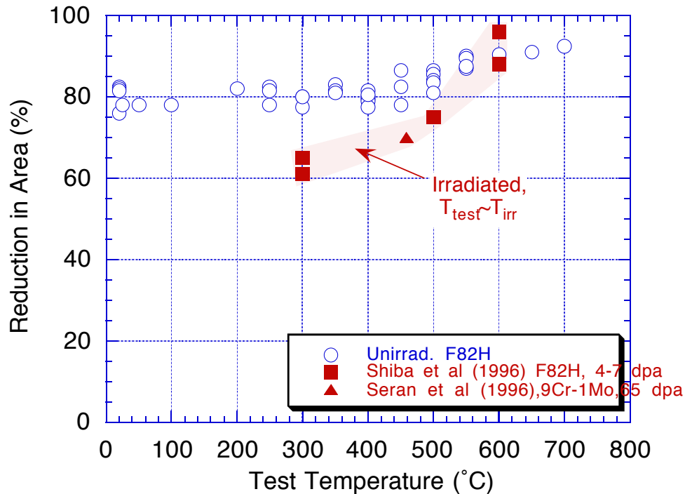
Fig. 6. Reduction in area of unirradiated and irradiated 8-9%Cr steels [1,3,5,6].
