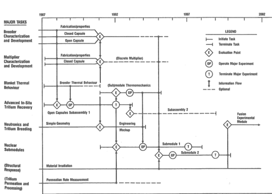
FIG. 7. Test sequence for major solid breeder blanket tasks.
