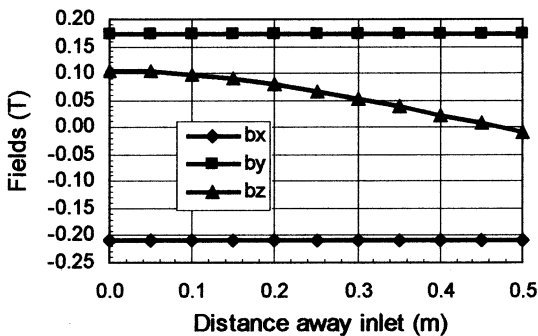
Fig. 1. NSTX outbound midplane 3D magnetic fields vs. x ( x denotes poloidal direction, y , toroidal and z , radial).
