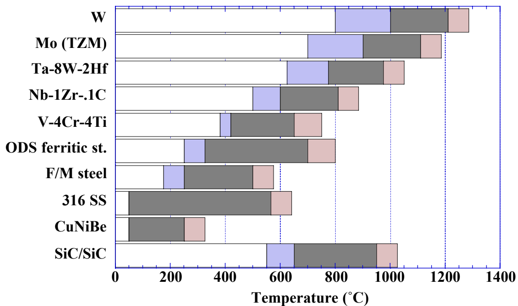
Fig. 6. Operating temperature windows (based on radiation damage and thermal creep considerations) for refractory alloys, Fe-(8-9%)Cr ferritic-martensitic steel, Fe-13%Cr oxide dispersion strengthened ferritic steel, Type 316 austenitic stainless steel, solutionized and aged Cu-2%Ni-0.3%Be, and SiC/SiC composites. The light shaded bands on either side of the dark bands represent the uncertainties in the minimum and maximum temperature limits.
