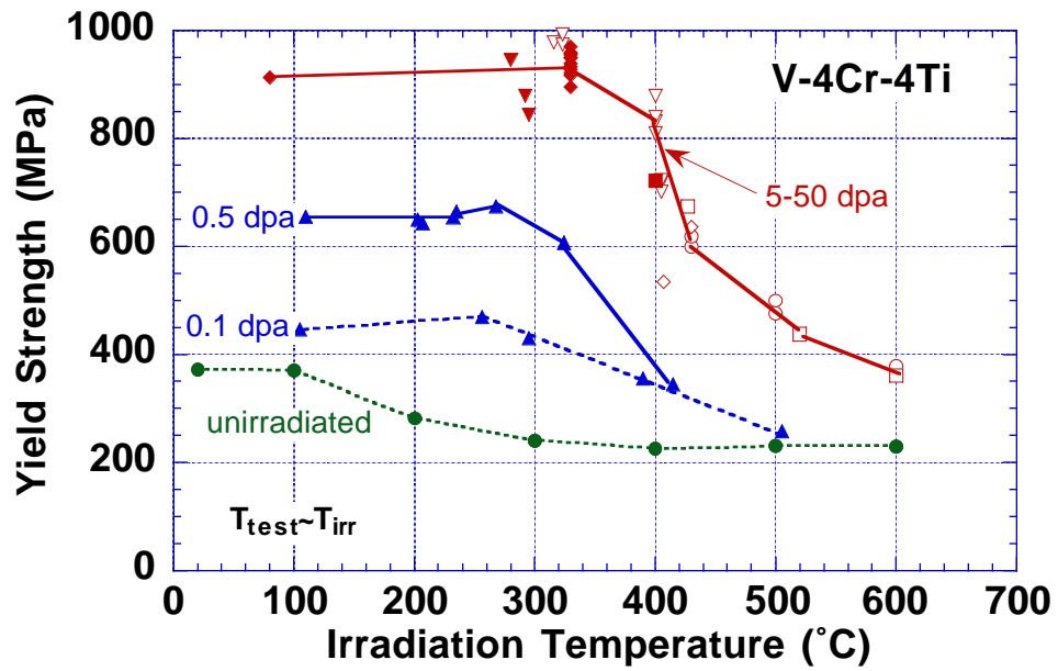
Fig. 3. Effect of irradiation temperature and dose on the yield strength of V-4Cr-4Ti [31,45].
