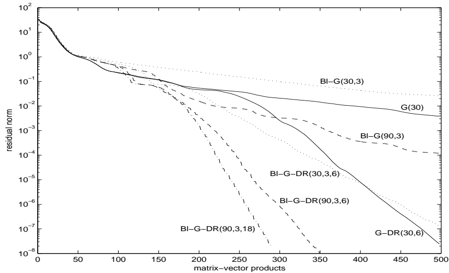
FIG. 4.1. Comparison of convergence for Sherman4 matrix.
