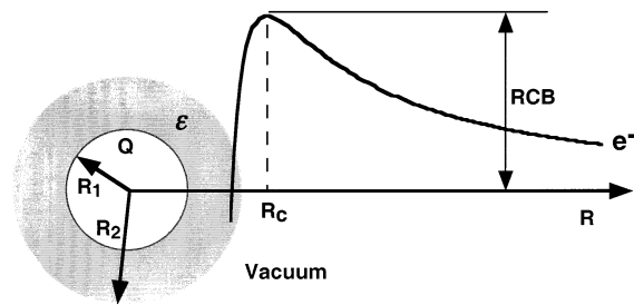
Figure 12. Electrostatic model used to calculate the RCB for detaching an electron from \text{SO}_4^{2-} in \text{SO}_4^{2-}(\text{H}_2\text{O})_n . The \text{SO}_4^{2-}(\text{H}_2\text{O})_n solvated clusters were modeled as a charged sphere (radius R_1 ) imbedded in a dielectric sphere (with radius R_2 , dielectric constant \epsilon ).
