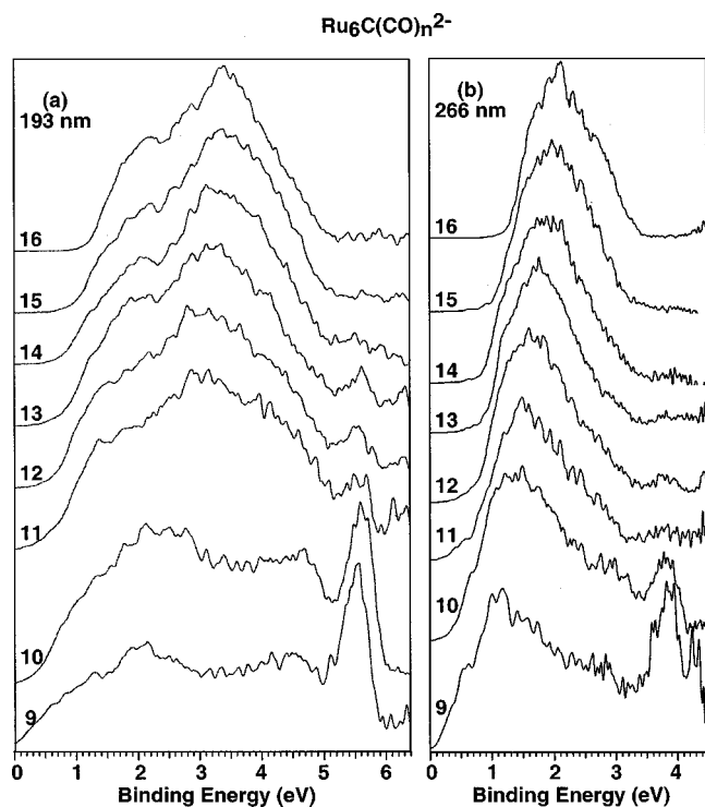
FIG. 4. Photoelectron spectra of \text{Ru}_6\text{C}(\text{CO})_n^{2-} ( n=9-16 ) at (a) 193 nm and (b) 266 nm (4.661 eV).
