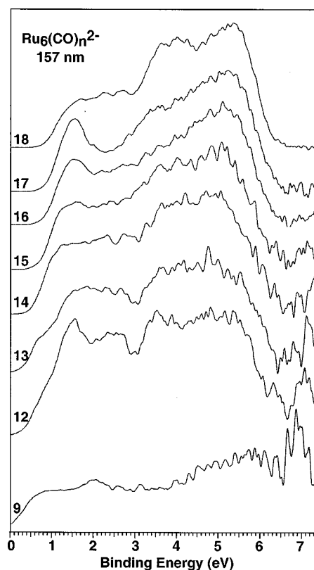
FIG. 5. Photoelectron spectra of \text{Ru}_6(\text{CO})_n^{2-} ( n=9-18 ) at 157 nm (7.866 eV).
