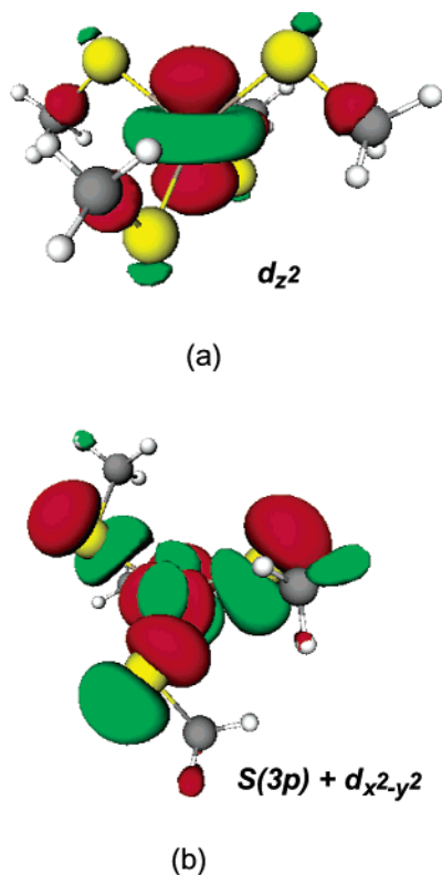
Figure 5. Molecular orbitals of (a) the reduced orbital ( d_{z^2} ) from [\text{Fe}(\text{SCH}_3)_4]^- to [\text{Fe}(\text{SCH}_3)_3]^- and (b) the oxidized orbital [\text{S}(3p) + d_{x^2-y^2}] from [\text{Fe}(\text{SCH}_3)_4]^- to [\text{Fe}(\text{SCH}_3)_3]^- .
