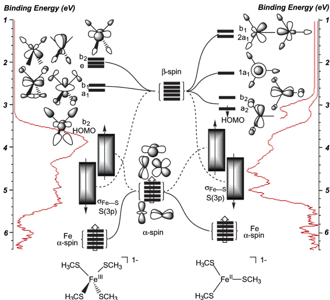
Figure 4. Schematic orbital interaction diagram for a tetrahedral D_{2d} [\text{Fe}(\text{SCH}_3)_4]^{1-} complex (the left-hand side) and a triangular C_{2v} [\text{Fe}(\text{SCH}_3)_3]^{1-} complex (the right-hand side) compared to the respective photoelectron spectra (red).
