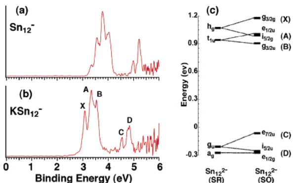
Figure 1. Photoelectron spectra of (a) \text{Sn}_{12}^- and (b) \text{KSn}_{12}^- at 193 nm. (c) Scalar relativistic (SR) energy levels of the 5p-based valence molecular orbitals of the I_h \text{Sn}_{12}^{2-} and the correlation to the spin-orbit (SO) coupled levels of I_h^* \text{Sn}_{12}^{2-} , where the asterisk indicates the double-group symmetry. See Supporting Information for computational details.
