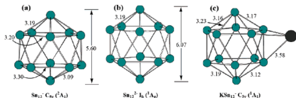
Figure 2. Optimized structures: (a) \text{Sn}_{12}^- ; (b) \text{Sn}_{12}^{2-} ; (c) \text{KSn}_{12}^- . The bond distances and cage diameters are in Å. See Supporting Information for computational details.
