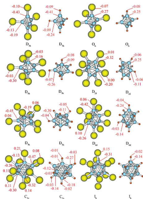
Figure 2. Calculated natural bond effective atomic charges in |e| (at B3LYP/LANL2DZ) for B_xH_x^{2-} and B_xAu_x^{2-} ( x = 5-12 ).
