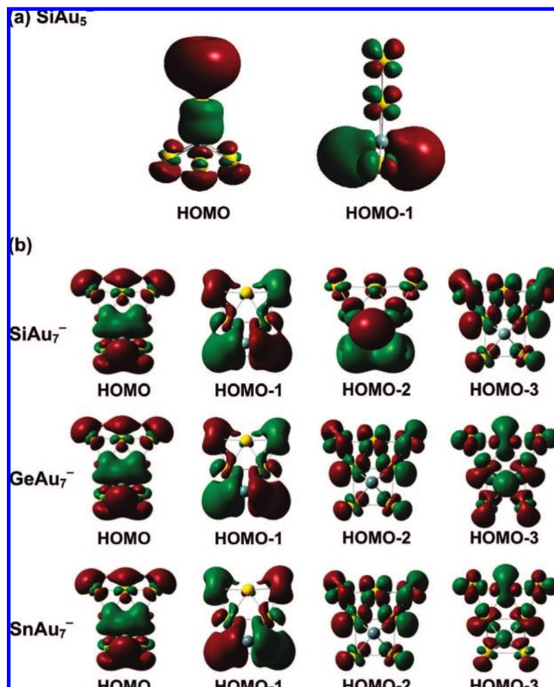
Figure 5. Selected frontier molecular orbitals of (a) SiAu 5 - and (b) MAu 7 - (M = Si, Ge, Sn).
