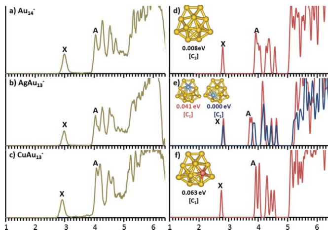
FIG. 2. Photoelectron spectra of Au_{14}^- , AgAu_{13}^- , and CuAu_{13}^- at 193 nm (left) compared with computed spectra and the cluster structures (right). Au—golden, Ag—blue, and Cu—red.
