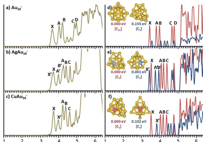
FIG. 3. Photoelectron spectra of Au_{15}^- , AgAu_{14}^- , and CuAu_{14}^- at 193 nm (left) compared with computed spectra and the cluster structures (right). Au—golden, Ag—blue, and Cu—red.
