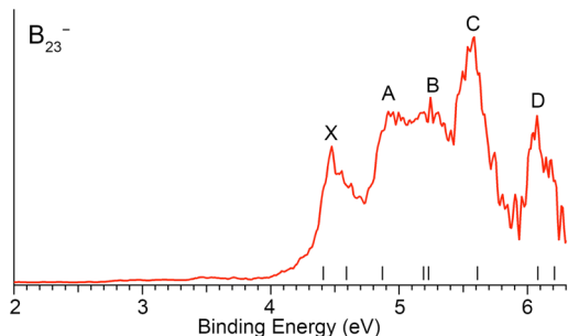
Figure 2. Photoelectron spectrum of B_{23}^- at 193 nm. Vertical bars represent calculated VDEs at the TD-PBE0/6-311+G(2df)//PBE0/6-311+G* level of theory. See Table 1.
