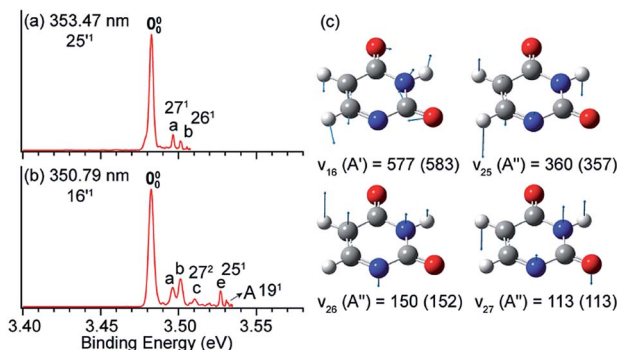
Fig. 9 Resonant PE spectra of [U-H]^- at (a) 353.47 nm and (b) 350.79 nm, corresponding to the DBS vibrational levels 25^{1/1} and 16^{1/1} , respectively. (c) The four relevant vibrational modes of the neutral radical [U-H] . The measured frequencies and the calculated values (within parentheses) are given in \text{cm}^{-1} . Adapted from ref. 5 with permission from Elsevier.
