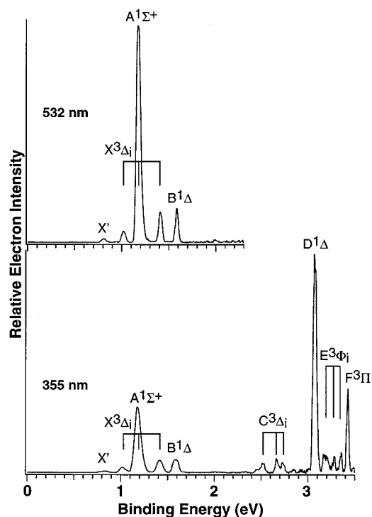
FIG. 2. Photoelectron spectra of WC - at 532 (2.331 eV) and 355 nm (3.496 eV) and their assignments.
