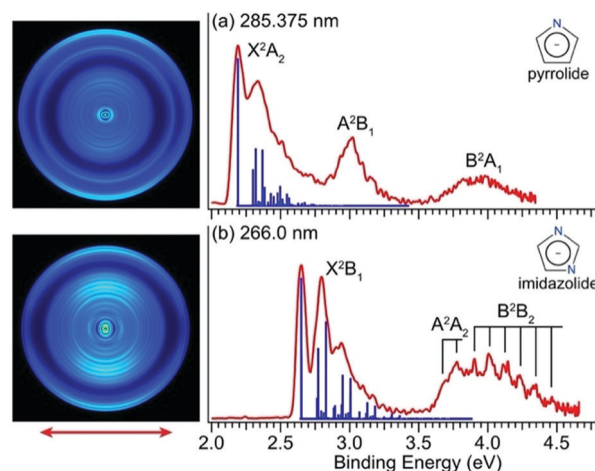
Fig. 1 PE images and spectra of (a) pyrrolide at 285.375 nm (4.3446 eV) and (b) imidazolidide at 266.0 nm (4.6611 eV). The calculated FC factors for the ground electronic states are represented as blue sticks for comparison. The insets display the molecular structures of the two anions. The double arrow below the images indicates the polarization direction of the detachment laser.
