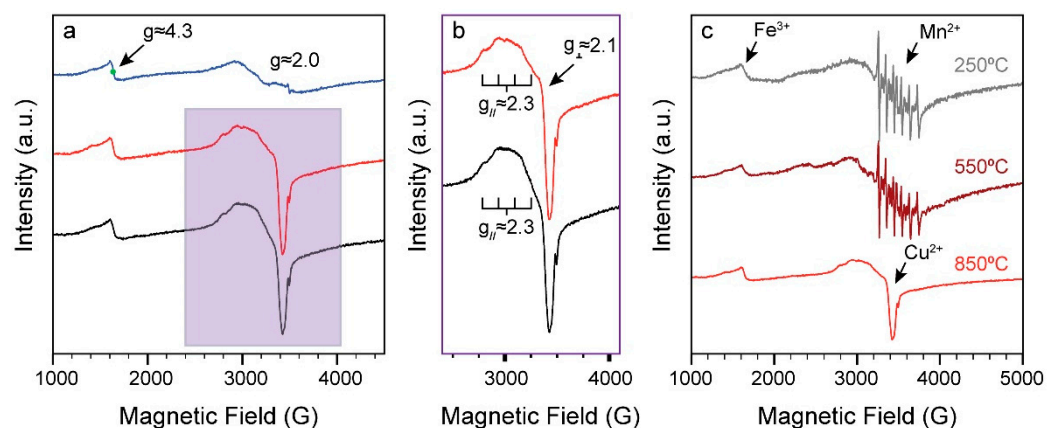
Figure 5. (a) EPR spectra for the no colorant (blue), 1% malachite (red), and 1% CuO (black) glazes fired to 850 °C. (b) Zoomed in EPR spectra for the 1% malachite (red) and 1% CuO (black) shown in the purple highlighted box in (a). (c) Normalized EPR spectra for the 1% malachite glaze series below 1000 °C (gray, dark red, and red fired to 250 °C, 550 °C, and 850 °C, respectively).
