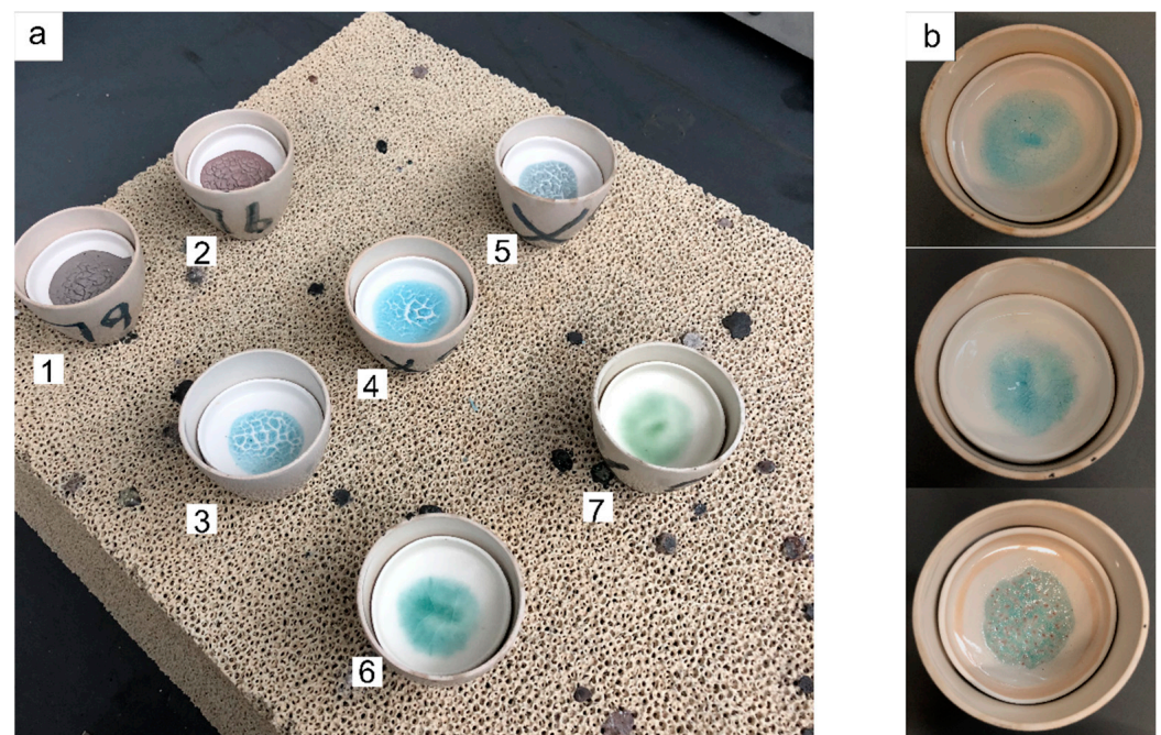
Figure 2. (a) Glazed crucible lids were prepared for 1% CuO (1) and 1% malachite (2) fired to 550 °C; 1% CuO (3), 1% malachite (4), and 1%CuO/1%SiC (5) fired to 850 °C, and the 1% CuO (6) and 1% malachite (7) glazes fired to 1000 °C directly taken out of the furnace, showing the initial green color. (b) Top to bottom: 1% malachite, 1% CuO, and 1% CuO/1% SiC glazes fired to 1000 °C in crucible lids following cooling.
