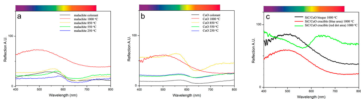
Figure 3. (a) Reflectance spectra for commercial malachite and the 1% malachite glaze series. (b) FORS reflectance spectra for CuO nanopowder and the 1% CuO glaze series. (c) Reflectance spectra for final 1% CuO/1% SiC glazes on different objects and in different areas.
