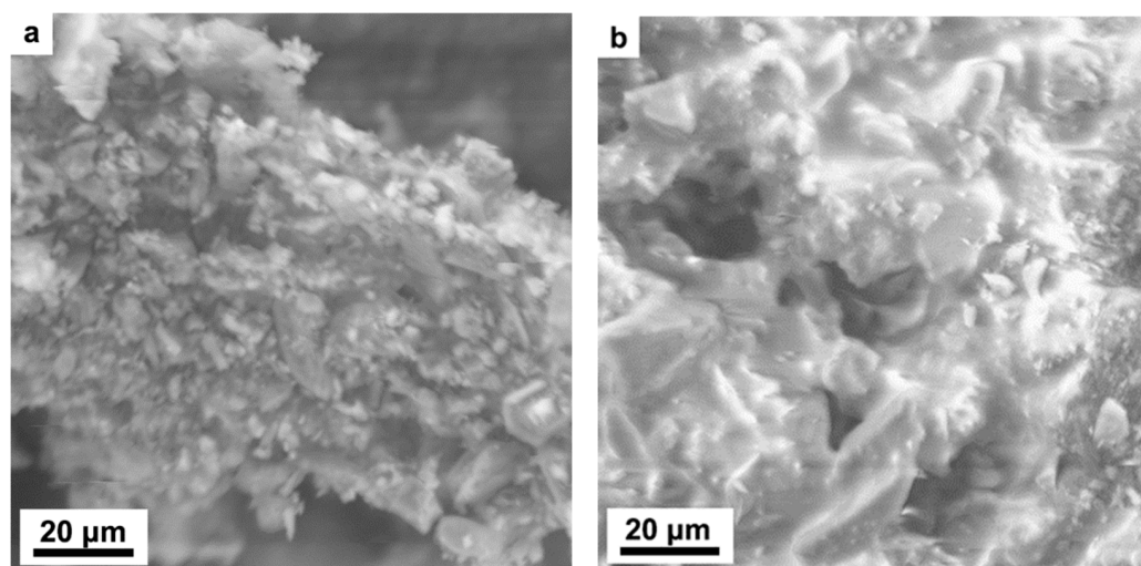
Figure 4. (a) SEM image for the 1% CuO glaze fired to 550 °C compared to the (b) 1% CuO glaze fired to 850 °C.
