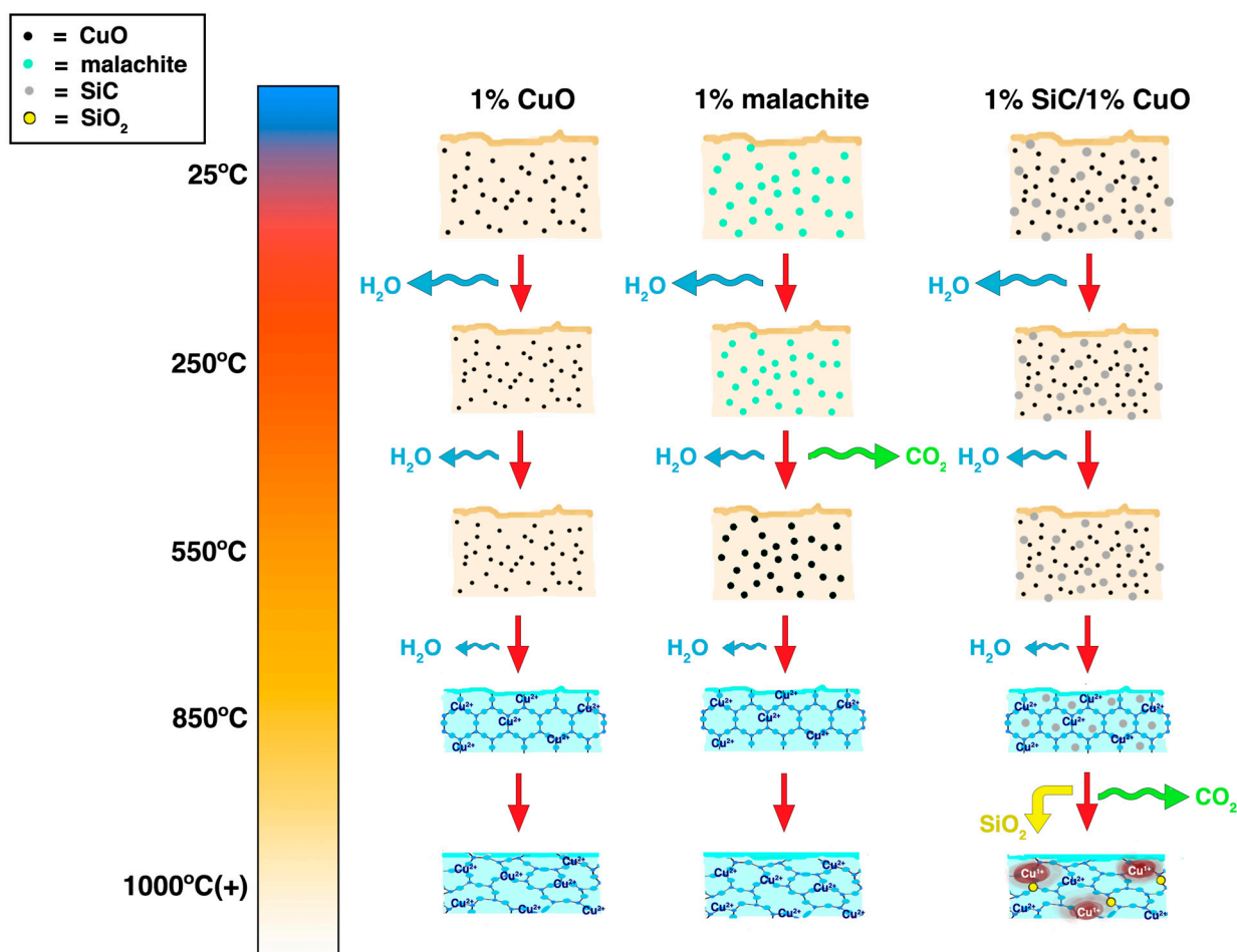
Figure 6. A schematic illustration showing the proposed mechanisms and timelines of the firing process for the “Robin’s egg blue” glaze variations. By 850 °C, the presence of color due to \text{Cu}^{2+} coordination suggests the presence of a silica-alumina matrix (represented by the regular ordered lattice structure), which becomes more disordered as the glaze becomes glass but ultimately still allows for coordination.
