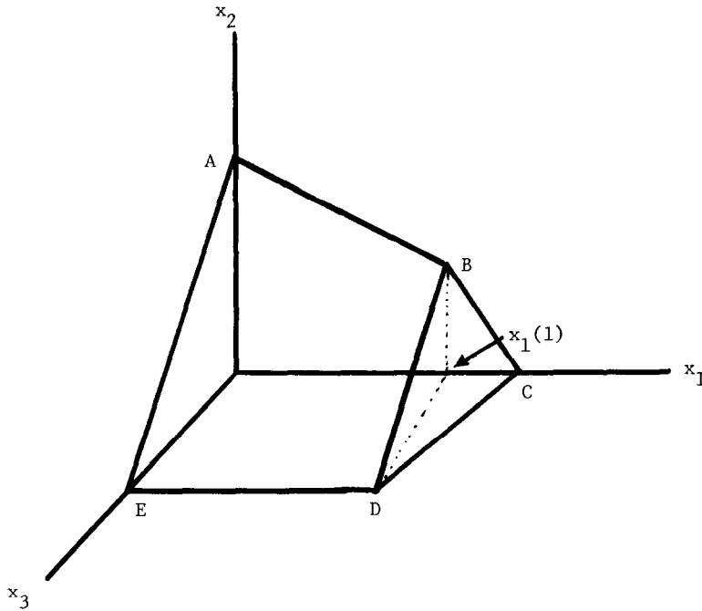
Fig. 1. Three-goods case with increasing block price on x_1 .
