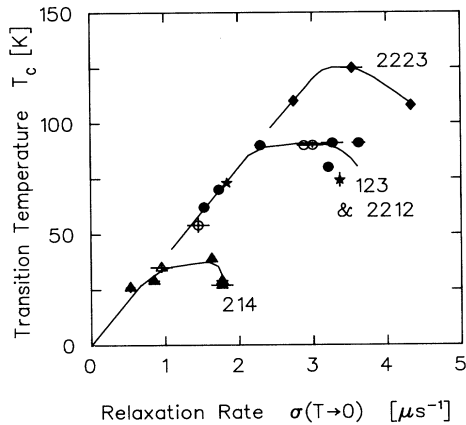
FIG. 2. The superconducting transition temperature T_c plotted vs low-temperature muon-spin-relaxation rate \sigma(T \rightarrow 0) measured in sixteen different specimens of CuO high- T_c superconductors. The horizontal axis \sigma(T \rightarrow 0) is proportional to 1/\lambda^2 and consequently to n_s/m^* . The closed triangles represent points for the 2:1:4 system \text{La}_{2-x}\text{Sr}_x\text{CuO}_4 , for x=0.08, 0.10, 0.15, 0.20, and 0.21 in the order of increasing \sigma . The first two points fall on the universal straight line. Closed circles denote the 1:2:3 systems \text{YBa}_2\text{Cu}_3\text{O}_y . In the order of increasing \sigma , points on the straight line are for y=6.67, 6.76, and 6.87 . The two closed circle points at around \sigma=3.1-3.5 with T_c=90 K are obtained for two different 1:2:3 specimens with y=7.0 . The closed circle at \sigma=3.2 and T_c=80 K represents (\text{Y}_{0.7}\text{Ca}_{0.3})\text{Ba}_2\text{Cu}_3\text{O}_7 . The two stars at T_c \sim 75 K represent the 2:2:1:2 and similar systems, \text{Bi}_2\text{Sr}_2\text{CaCu}_2\text{O}_8 and (\text{Tl}_{0.5}\text{Pb}_{0.5})\text{Sr}_2\text{CaCu}_2\text{O}_7 , in the order of increasing \sigma . The results for systems with triple CuO layers are shown by closed diamonds; \text{Bi}_{2-x}\text{Pb}_x\text{Sr}_2\text{Ca}_2\text{Cu}_3\text{O}_{10} , \text{Tl}_2\text{Ba}_2\text{Ca}_2\text{Cu}_3\text{O}_{10} , and (\text{Tl}_{0.5}\text{Pb}_{0.5})\text{Sr}_2\text{Ca}_2\text{Cu}_3\text{O}_9 , at T_c=110-125 K in the order of increasing \sigma . For the purpose of comparison, the four points reported in Ref. 19 are plotted by an open triangle ( \text{La}_{1.85}\text{Sr}_{0.15}\text{CuO}_4 ) and open circles ( \text{YBa}_2\text{Cu}_3\text{O}_y , with y=6.66, 6.95, and 7.0 in the order of increasing \sigma ). Note that these four points are obtained with experimental conditions and specimens different from those in the present measurements. Error bars are within the size of each point unless specified. Solid lines are guides to the eye.
