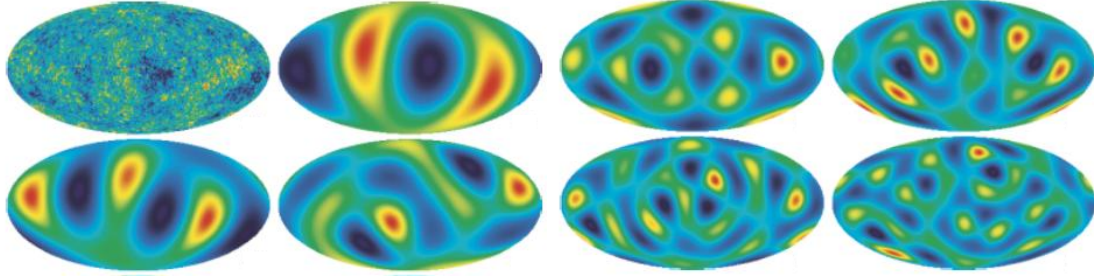
Figure 2.7: Representation of the multipole analysis of the CMB data. The multiple harmonics contribute differently to the thermal anisotropies. The analysis is made from lower multipoles excluding l = 0; 1 and up to higher multipoles of order l \approx 1000 . Higher multipole number l represents smaller angular distances between fluctuations. The first image is a representation of the CMB map, while the subsequent images are representations of the correlation function in terms of multipole moments, from l = 1 (dipole) to l = 7 . Figures from [Col15b].
