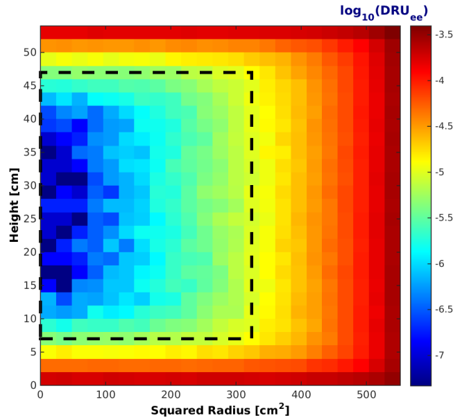
Figure 5.8: Simulated ^{127}\text{Xe} ER background density in the range 0.9 - 5.3 \text{ keV}_{ee} as a function of position, taken from the decay event density. Rates are in units of \log_{10}(\text{DRU}_{ee}) . The 118 kg fiducial volume used in the 85.3 day WIMP search run is overlaid as the black dashed contour.
