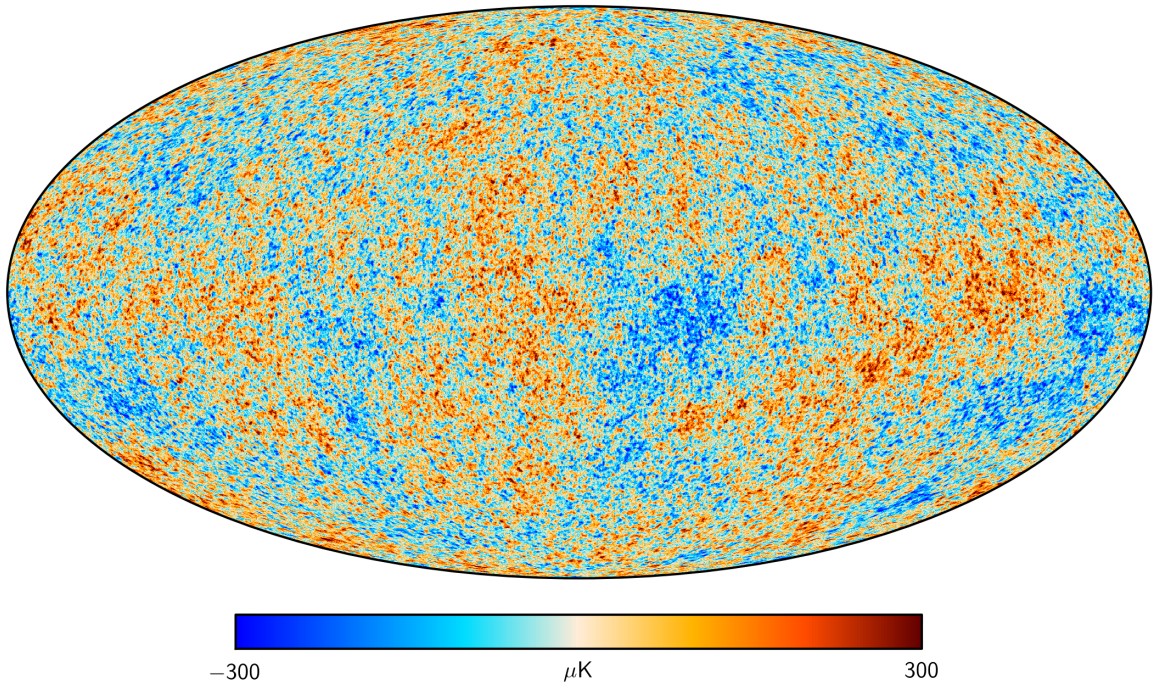
Figure 2.4: Mollweide projection of the CMB seen by the Planck satellite with the 2015 data, with monopole (mean temperature) and dipole (Doppler shift) contributions removed. Figure taken from [Col15b].
