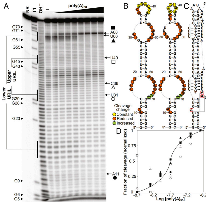
Fig. 6. In-line probing analyses of the wild-type dENE. (A) In-line probing analyses of 32 P 5' end-labeled dENE in the absence (—) and presence of varying concentrations of poly(A) (2 to 320 nM) at room temperature (22 °C). Lane NR shows no reaction, lane T1 indicates RNase T1-digested RNA (G-specific cleavage), and lane OH - shows alkaline-mediated partial digestion. (B) Sequence and secondary structure models for the wild-type dENE (derived from in-line probing data in the absence of poly(A) on the Left and the predicted from comparative sequence analysis (11) on the Right ). Nucleotide linkages that undergo constant, reduced, or increased cleavage upon poly(A) binding as determined by their relative band intensities in A are circled in yellow, red, or green, respectively. (C) Schematic of the poly(A)-bound dENE structure derived from the crystal structure (14). Long-range interactions between the A-triad nucleotides (boxed in red) are indicated by solid gray lines. (D) Dependence of the fraction of cleavage at selected sites (marked in A) in the lower dENE domain (closed symbols) and the upper dENE domain (open symbols) on poly(A) concentration. Calculation of fraction modulated is described in Materials and Methods . Data from selected cleavage sites were plotted against the logarithm of poly(A) concentration showing an apparent K D of ~15 to 30 nM. The solid line indicates a theoretical binding curve for a 1:1 dENE-poly(A) interaction with a K D of 20 nM.
